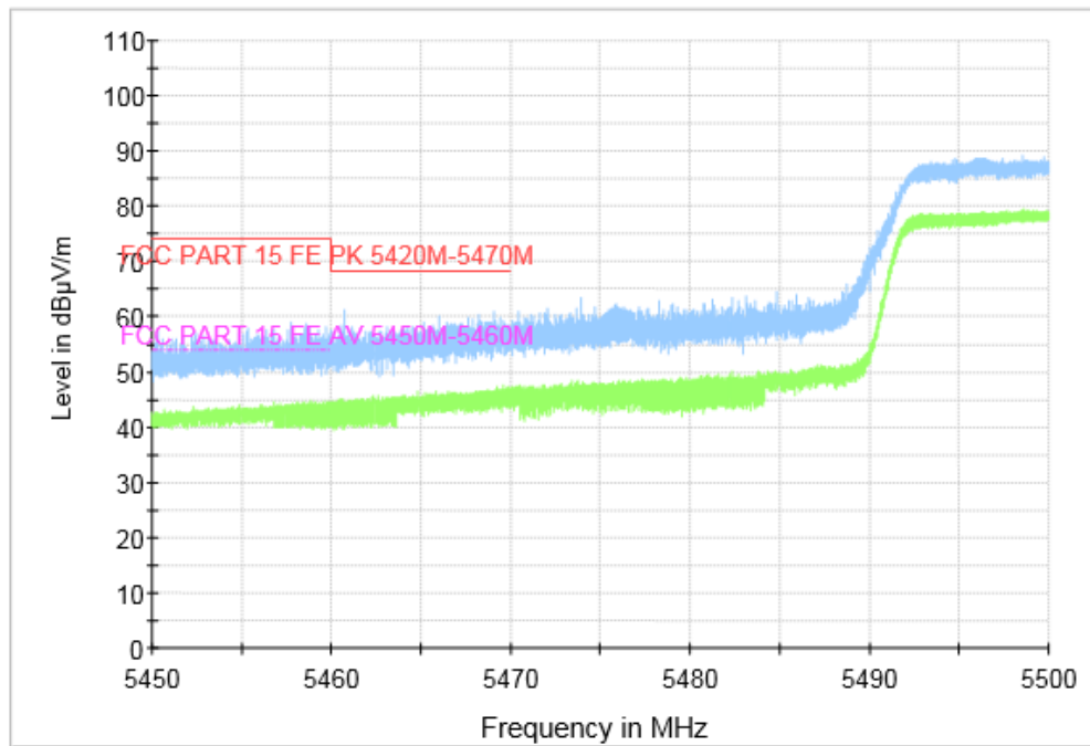
Fig. 61 Band Edges (802.11ac-VHT80, CH106 5530MHz)
