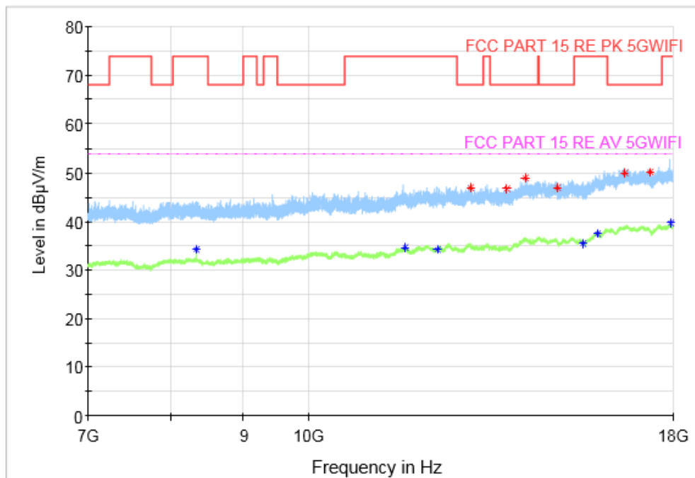
Fig. 106 Transmitter Spurious Emission (802. 11ac-VHT80, CH42 5210MHz, 7 GHz-18 GHz)
