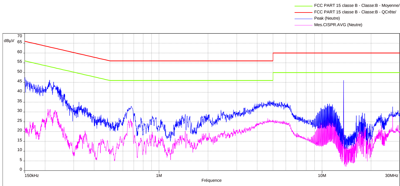
Diagram N°4 Mode DC Neutral 120/60Hz
