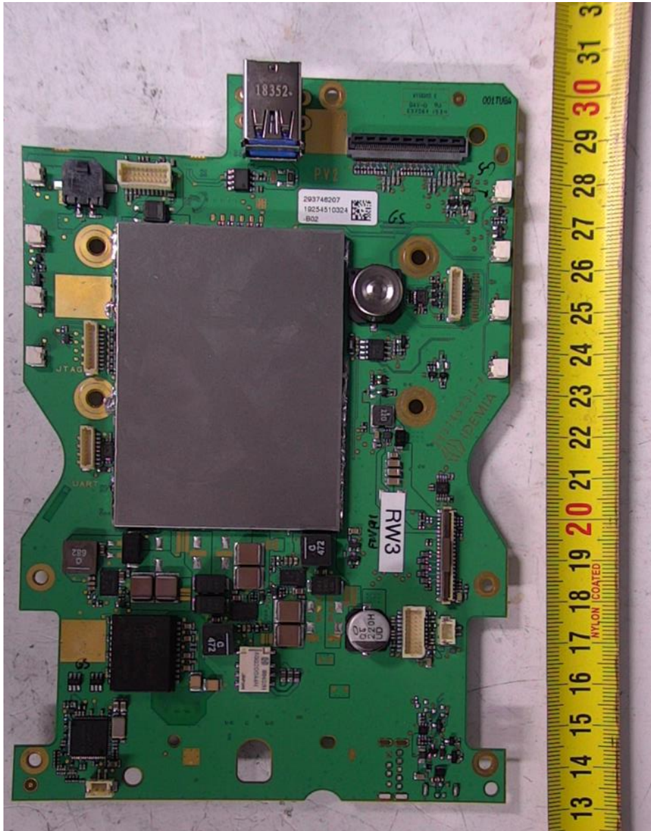
MB board Top view (with shielding)
