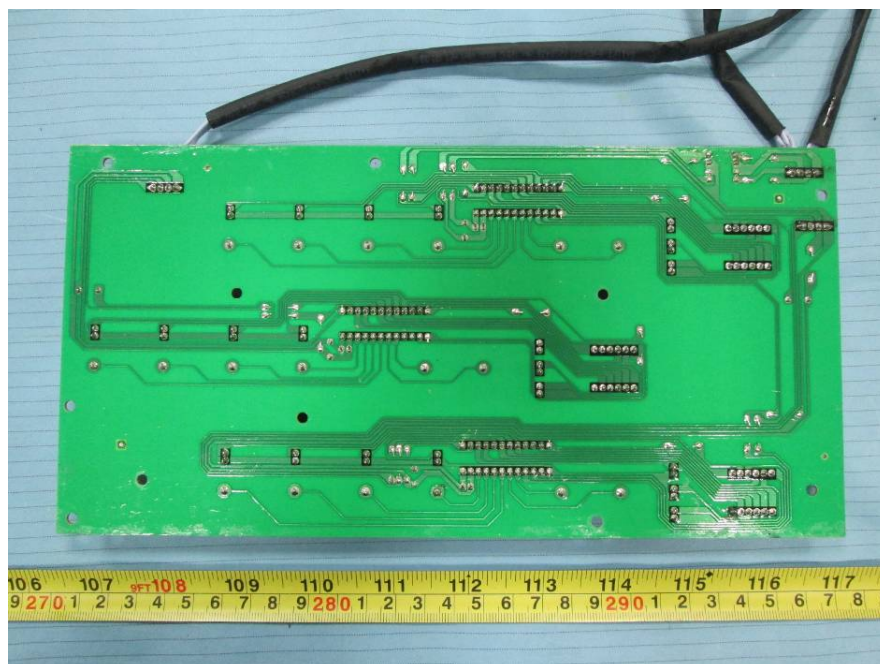
EUT –Control Pannel Main Board Bottom View
