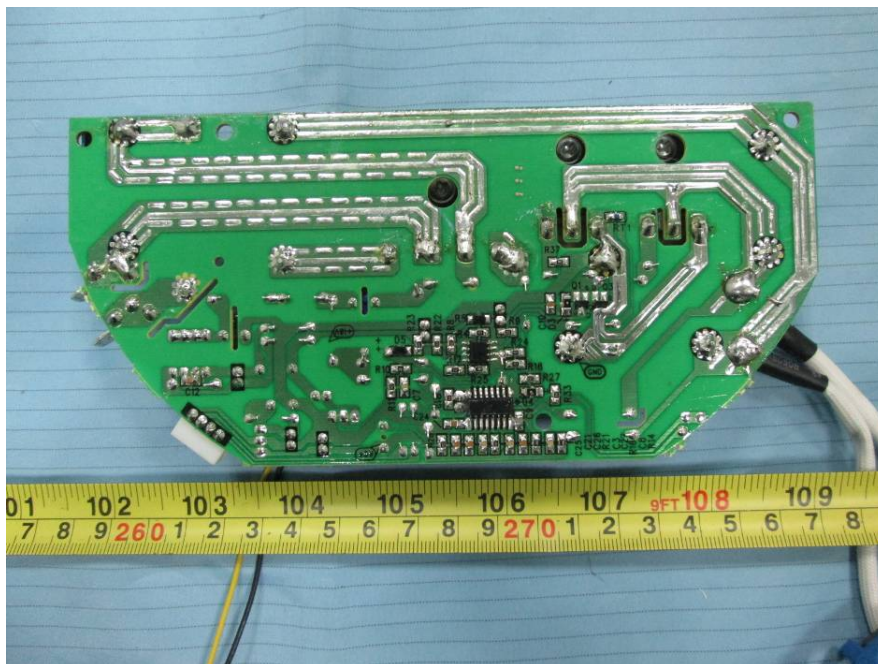
EUT – Electromagnetic Coil Main Board Bottom View
