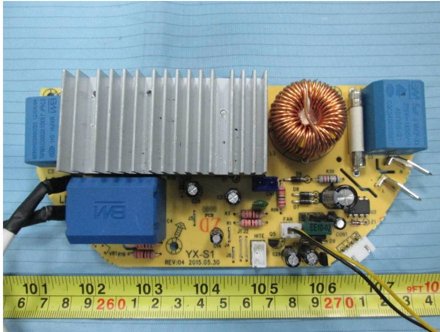
EUT – Electromagnetic Coil Main Board Top View
