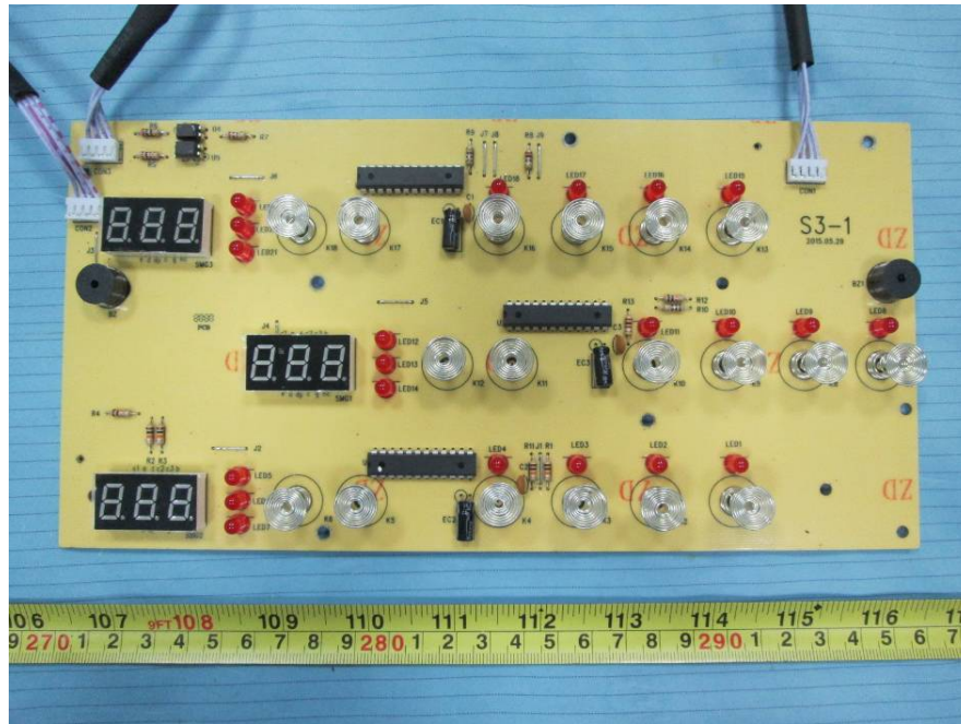
EUT – Control Pannel Main Board Top View
