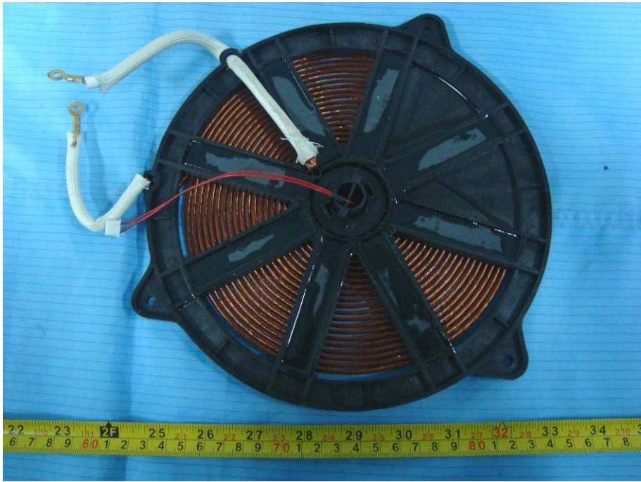
EUT – Induction Coil Rear View
