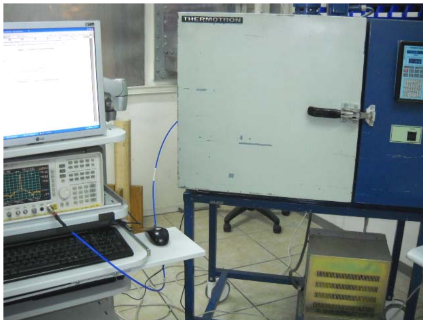
Photograph No.5 Setup for frequency stability test
