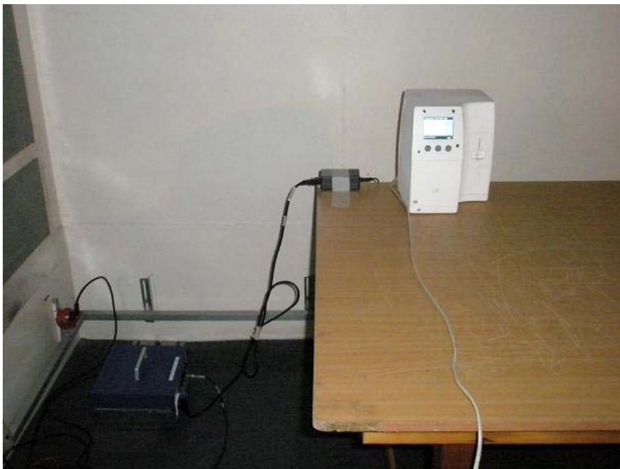
Photograph No.8 Setup for conducted emission measurements in shielded room
