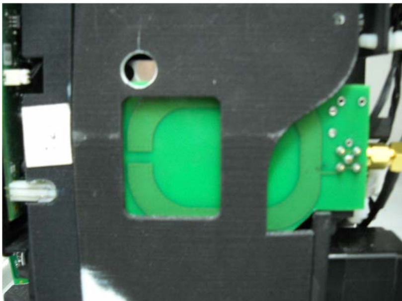
Photograph No.2 Antenna placement in the Scanner
