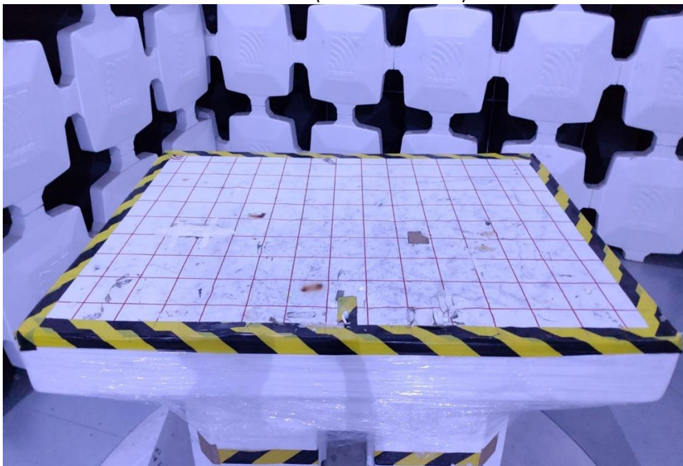
Back View (30MHz to 1GHz)
