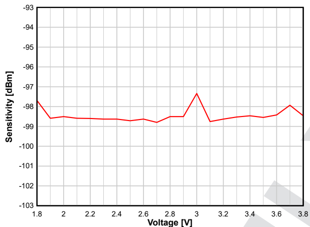
Figure 8-20. Sensitivity vs. Supply Voltage (VDDS) (250 kbps, 2.44 GHz)
