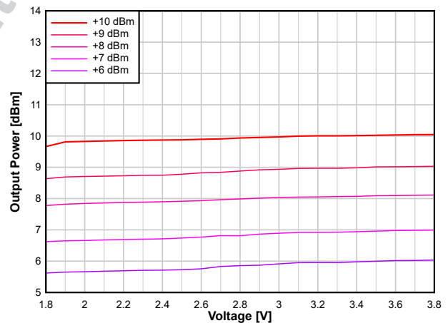
Figure 8-26. Output Power vs. Supply Voltage (VDD5) (2.44 GHz, +10 dBm PA)
