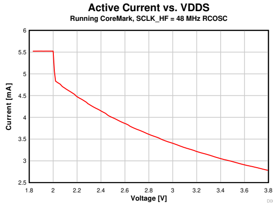
Figure 8-4. Active Mode (MCU) Current vs. Supply Voltage (VDD) (Running CoreMark, SCLK_HF = 48 MHz RCOSC)
