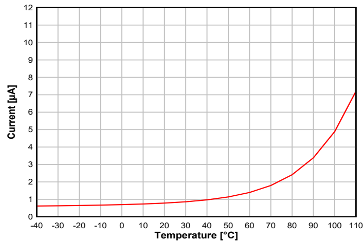
Figure 8-6. Standby Mode (MCU) Current vs. Temperature, 80kB RAM retention, no Cache retention, RTC On SCLK_LF = 32 kHz XOSC, VDD = 3.6 V
