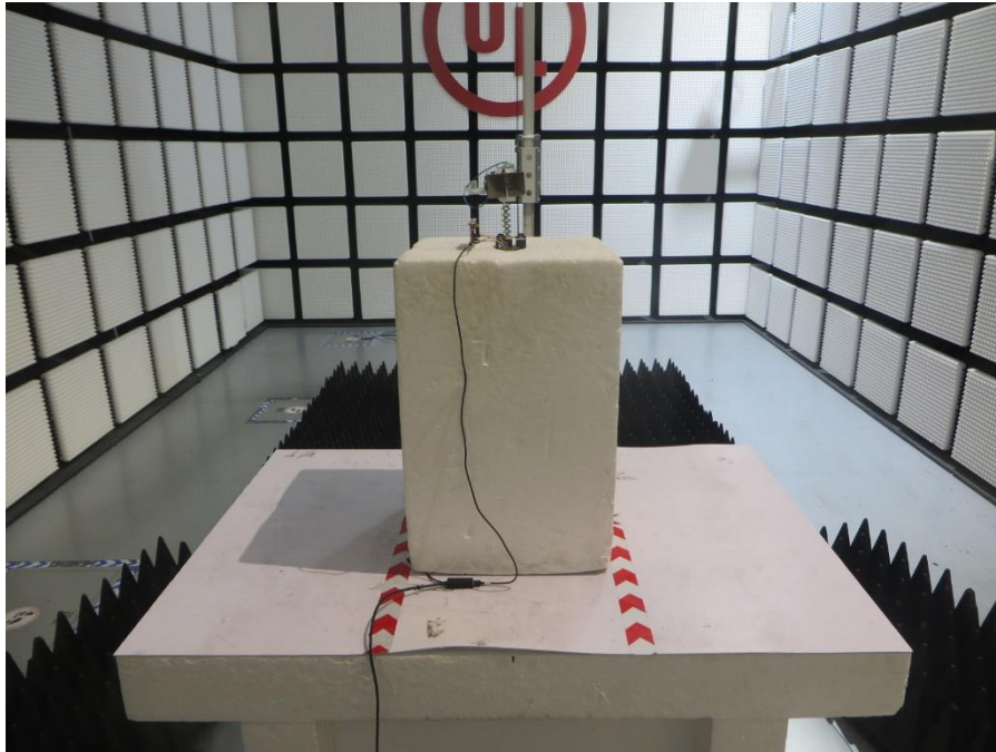
MEASUREMENT POSITION (X axis) ---condition 3
