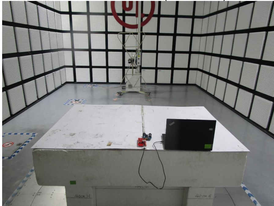
RADIATED RF MEASUREMENT SETUP (Below 30MHz) ---condition 3
