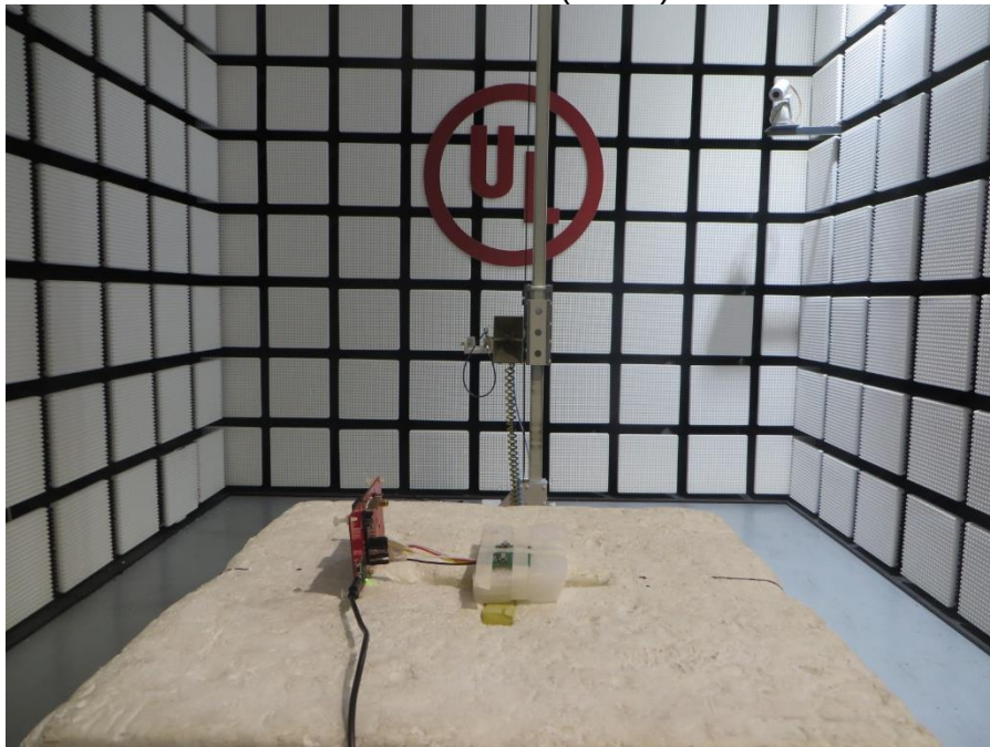
MEASUREMENT POSITION (X axis) ---condition 1
