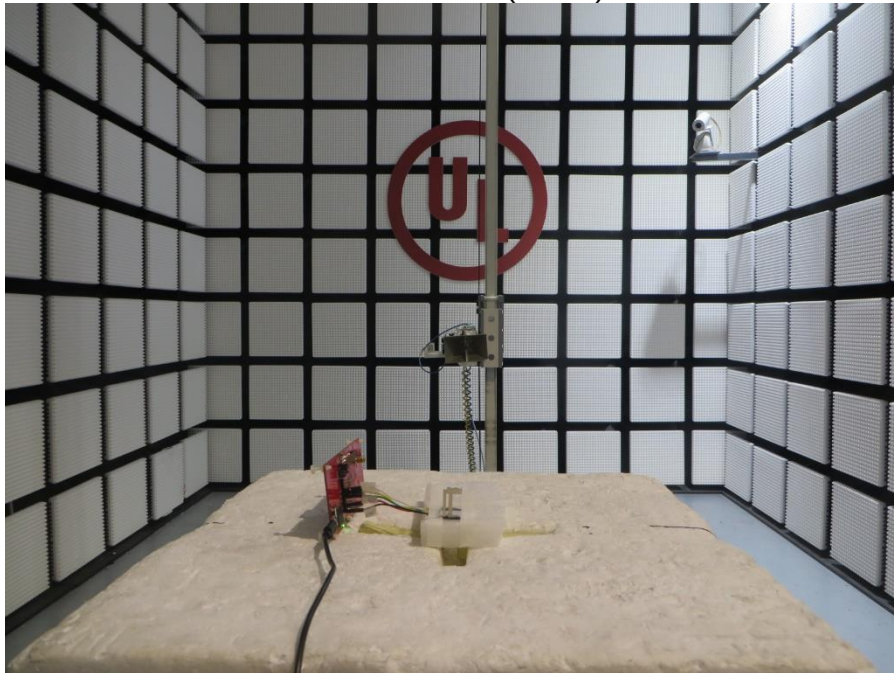
MEASUREMENT POSITION (X axis) ---condition 2
