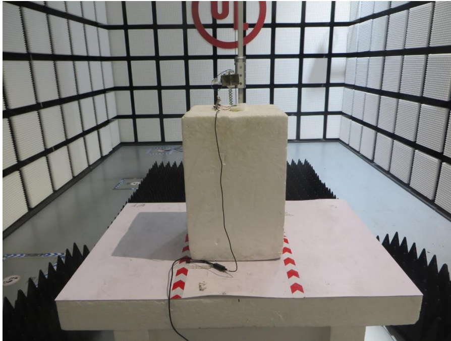
MEASUREMENT POSITION (X axis) ---condition 5
