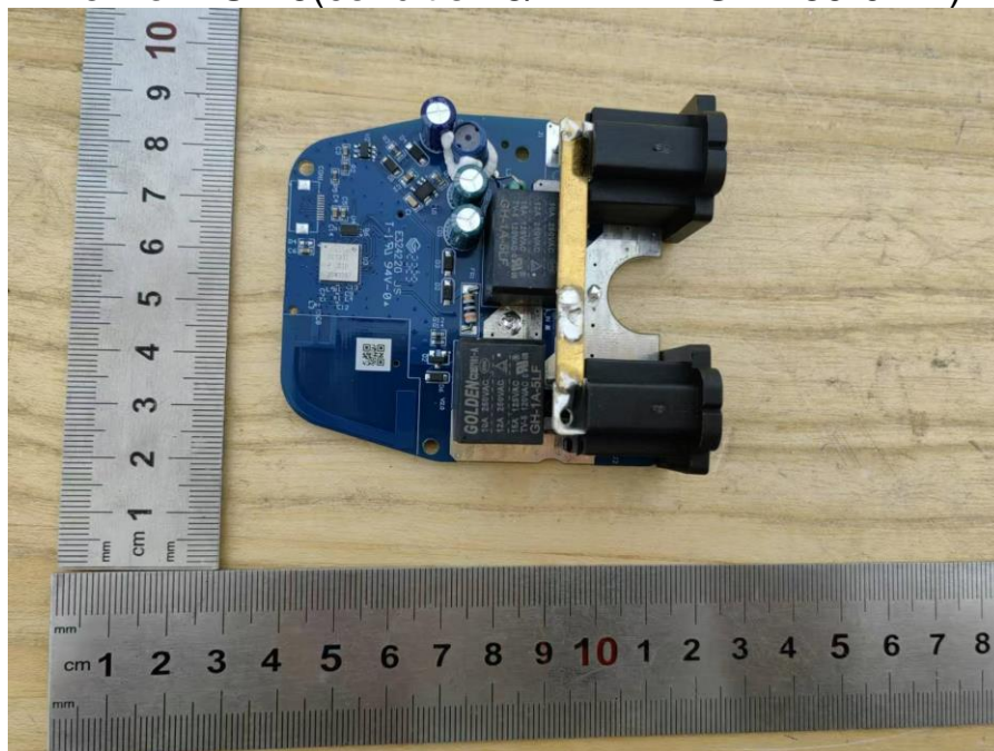
View of EUT-6(condition 3/HVIN: D-SP-A39-02-A)
