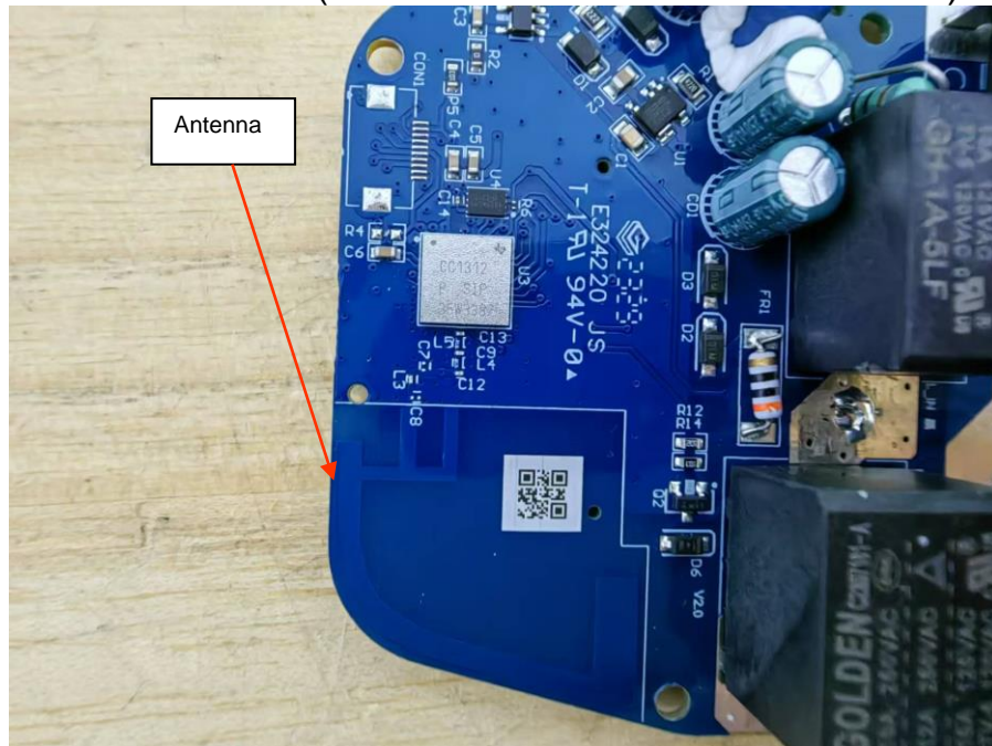
View of EUT-7(condition 3/HVIN: D-SP-A39-02-A)
