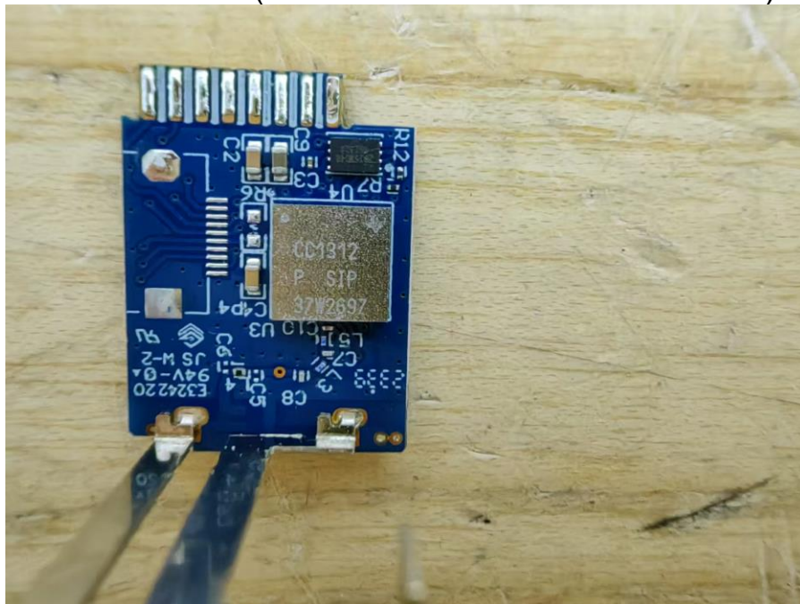
View of EUT-4(condition 2/HVIN: D-SP-A46-01-A)
