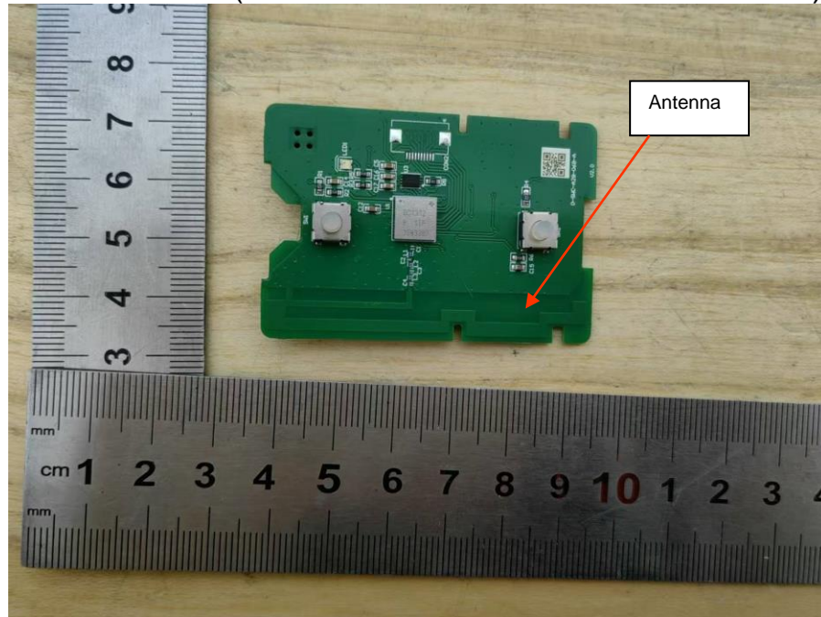
View of EUT-1(condition 1/HVIN: D-SWC-A28-06B-A)
