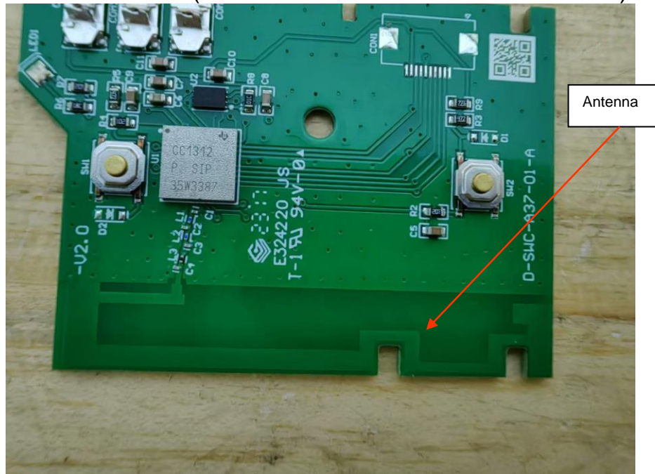
View of EUT-13(condition 5/HVIN: D-SWC-A37-01-A)
