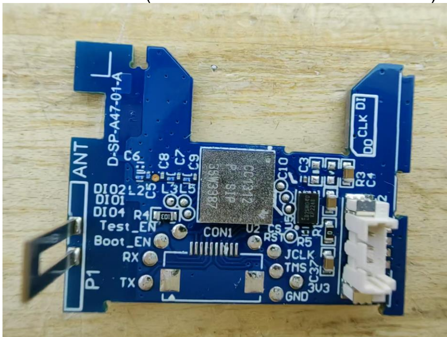
View of EUT-10(condition 4/HVIN: D-SP-A47-01-A)
