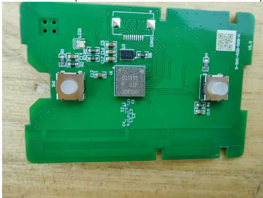
View of EUT-2(condition 1/HVIN: D-SWC-A28-06B-A)
