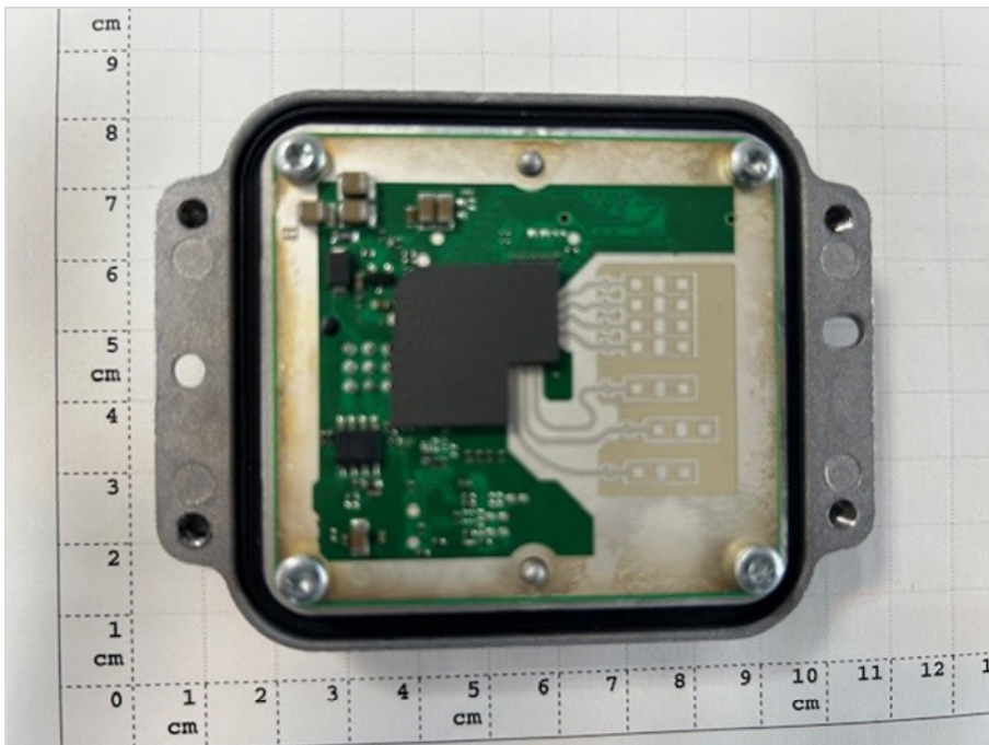
Photograph 6: EUT 2_Inside view 3
