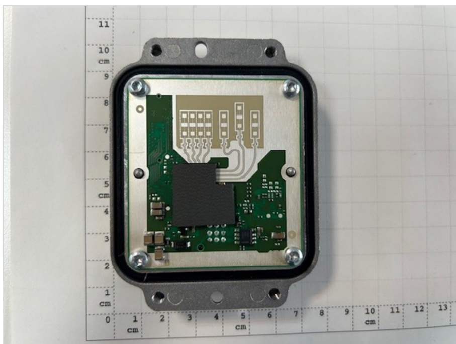
Photograph 8: EUT 3_Inside view 2
