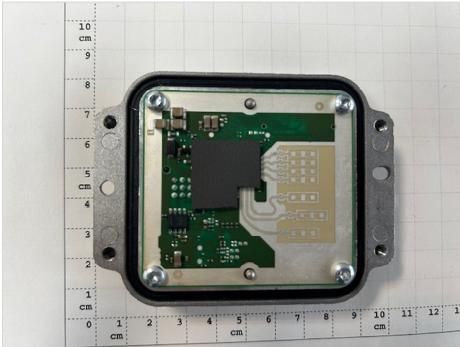
Photograph 9: EUT 3_Inside view 3
