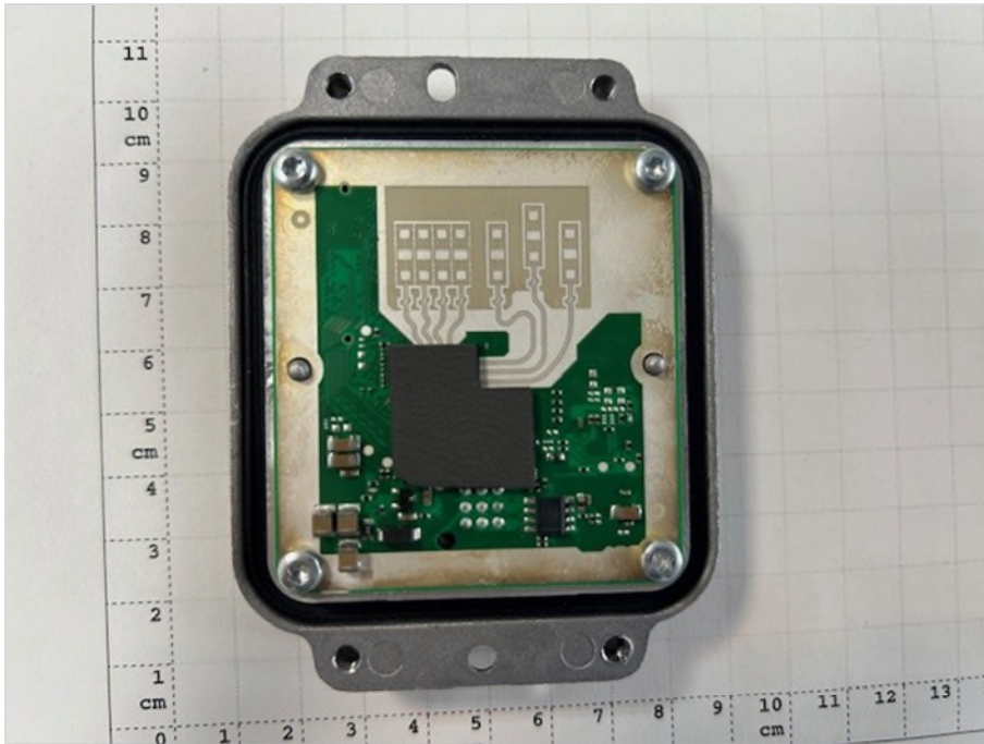
Photograph 5: EUT 2_Inside view 2
