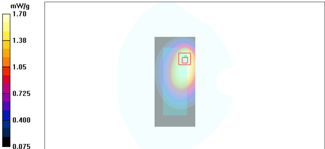
Figure 14 Body-Worn, Back Towards Ground for 12.5KHz 450.125 MHz
