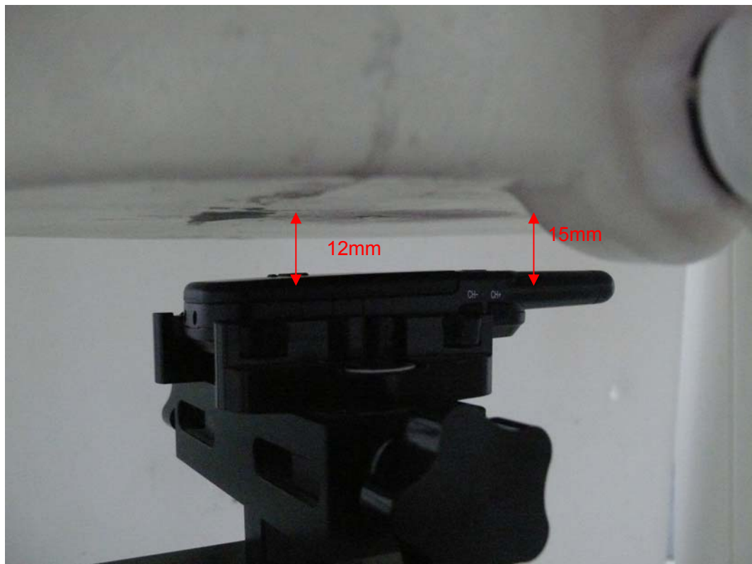
Picture 5: Body-worn, The EUT display towards ground, Belt clip attach the Phantom, the distance from EUT Antenna to the bottom of the Phantom is 15mm
