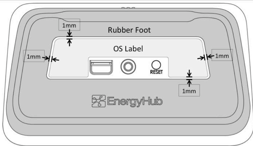
OS Label Location on the Home Base – Bottom View
