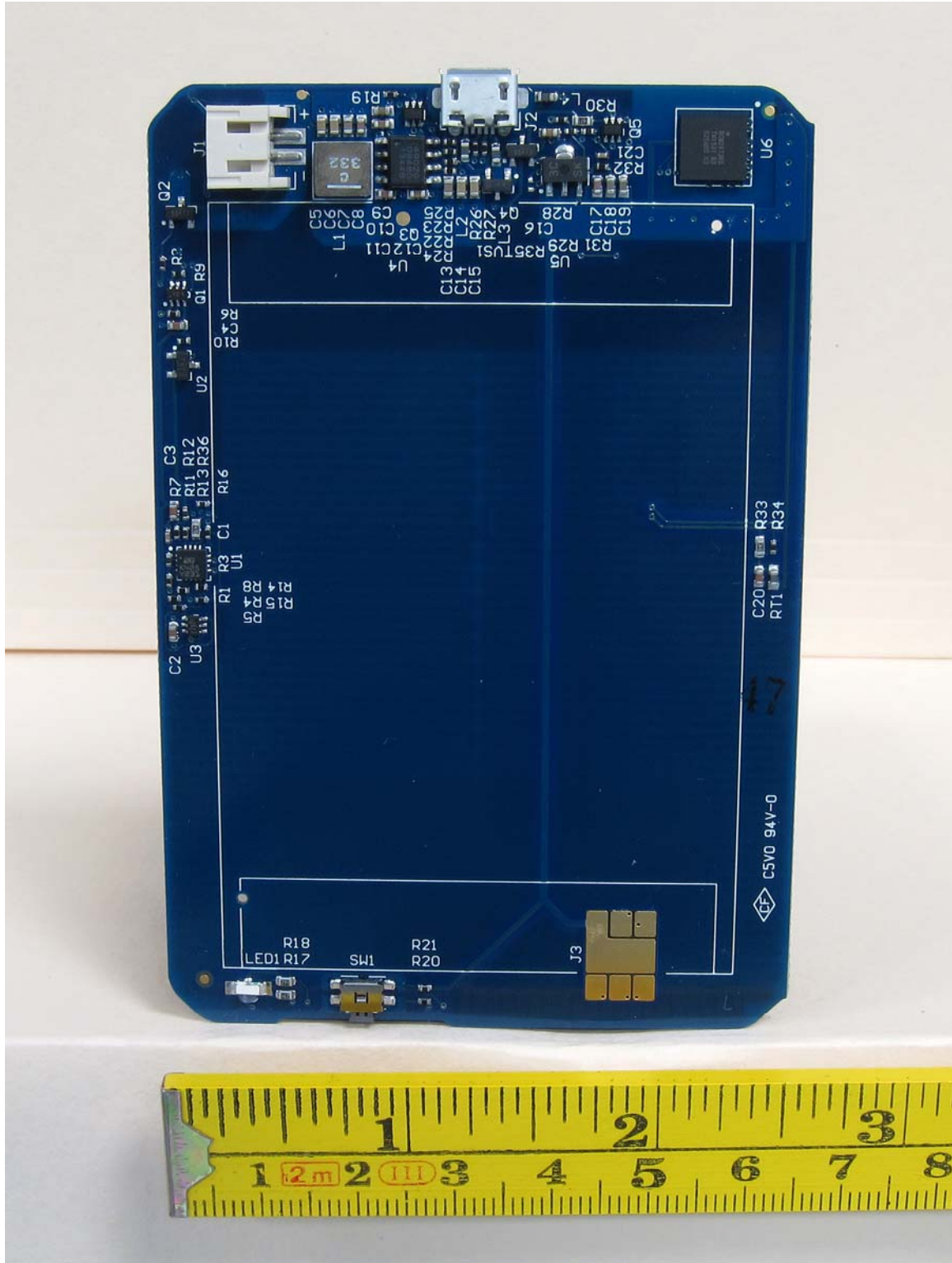
PCB Front
