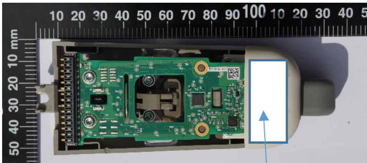
Photo : UI-Joystick module Bottom view, including location of label
