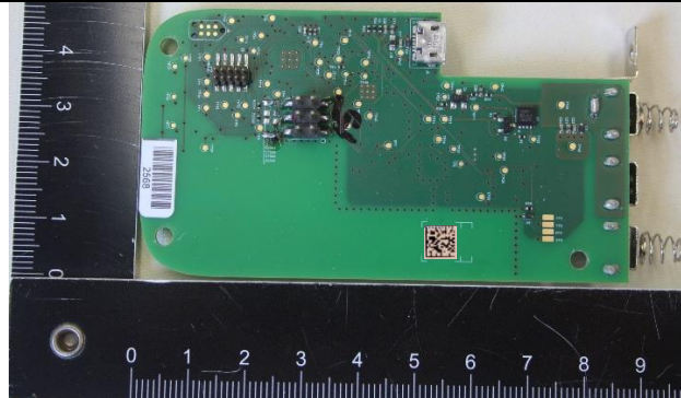
Photo 2: Remote Control PCB Bottom view
