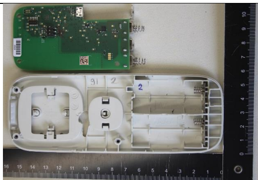
Photo 3: PCBA and housing
