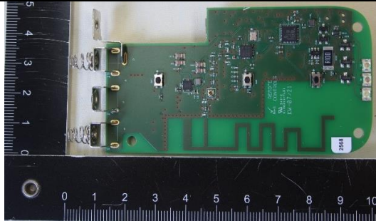
Photo 1: Remote Control PCBA Top view
