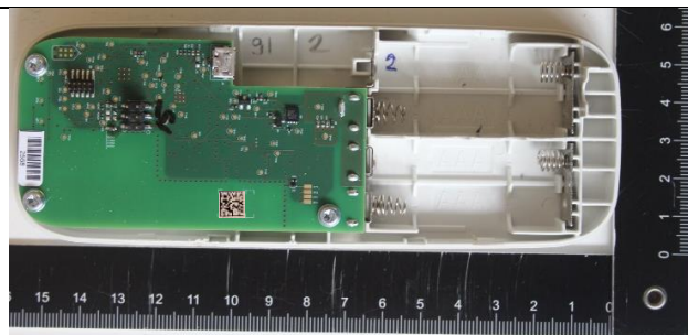
Photo 2: Remote Control PCB Bottom view
