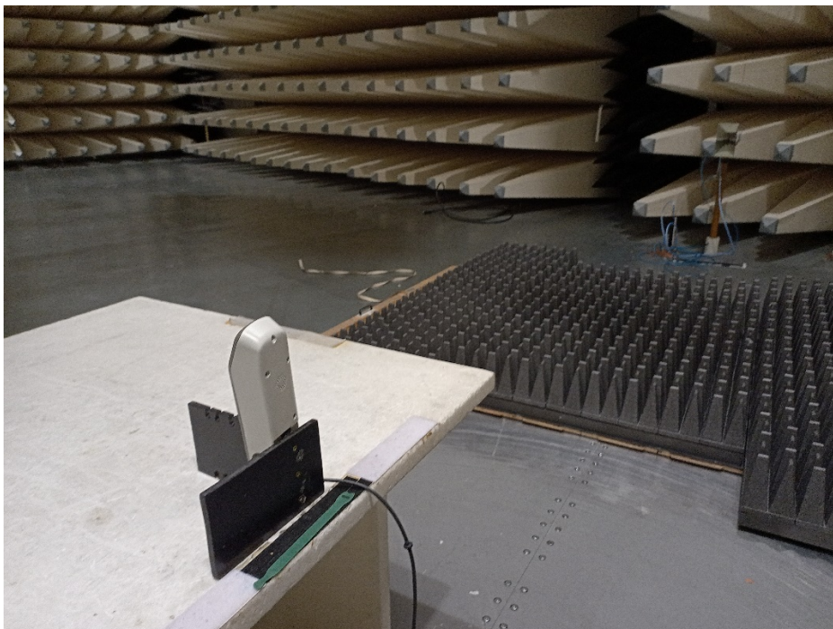
Photo 2: Radiated Emission
