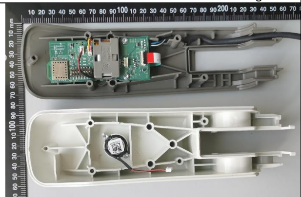
Photo 7: 1122596 Call module device open top/bottom
