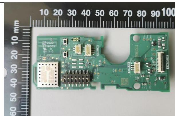
Photo 2: 1122596 Call module PCBA Bottom view
