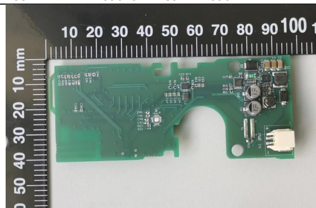
Photo 1: 1122596 Call module PCBA Top view
