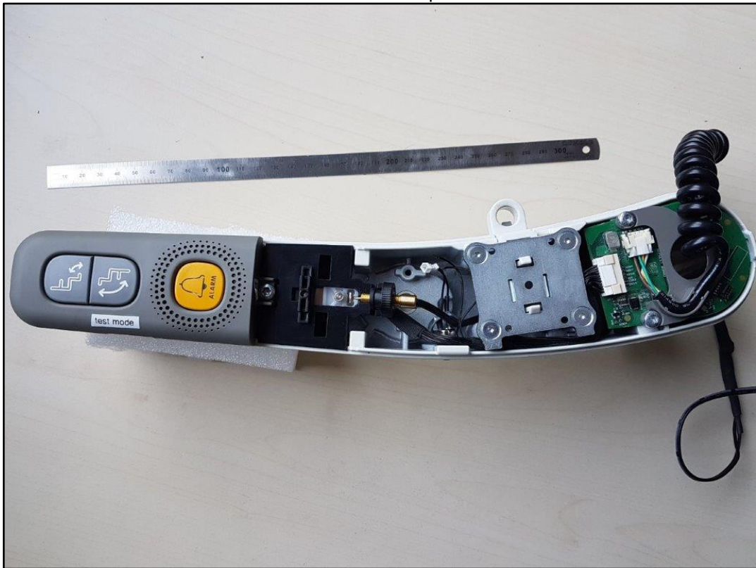
Photo 6: DUT - top side
