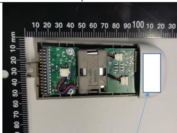
Photo 1: 1060661 Call module PCBA Top view
