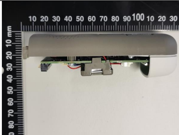
Photo 7: 1060661 Call module device side right
