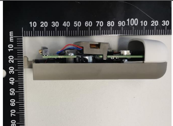
Photo 8: 1060661 Call module device side left
