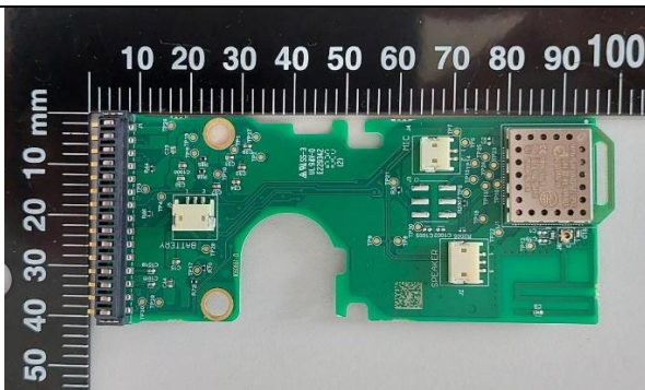
Photo 2: 1060661 Call module PCBA Bottom view
