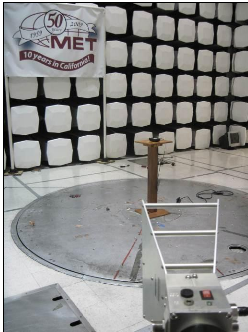
Photograph 7. Radiated Emission, Test Setup, 1 GHz – 10 GHz
