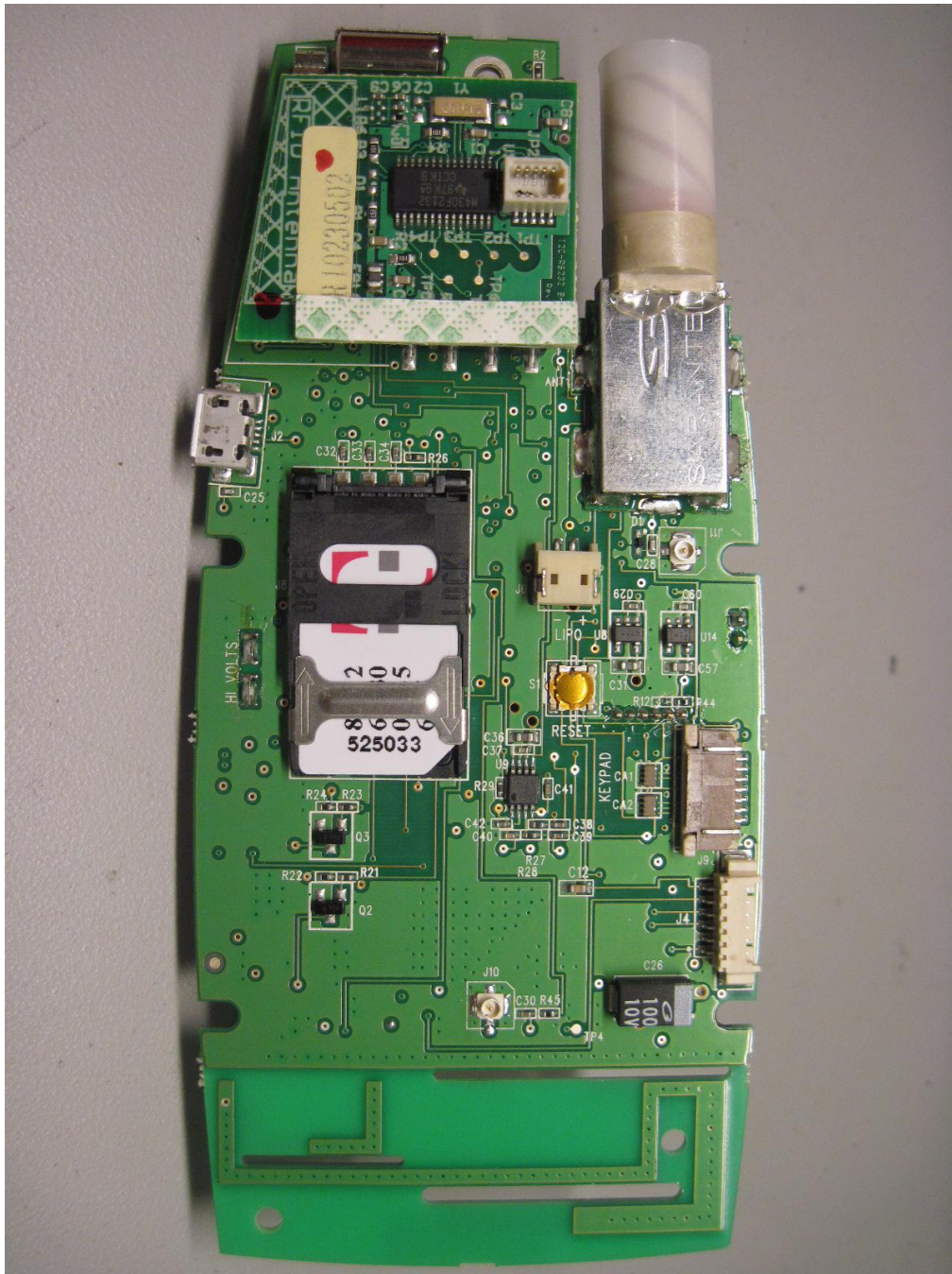
Photograph 2. EUT Board Read View
