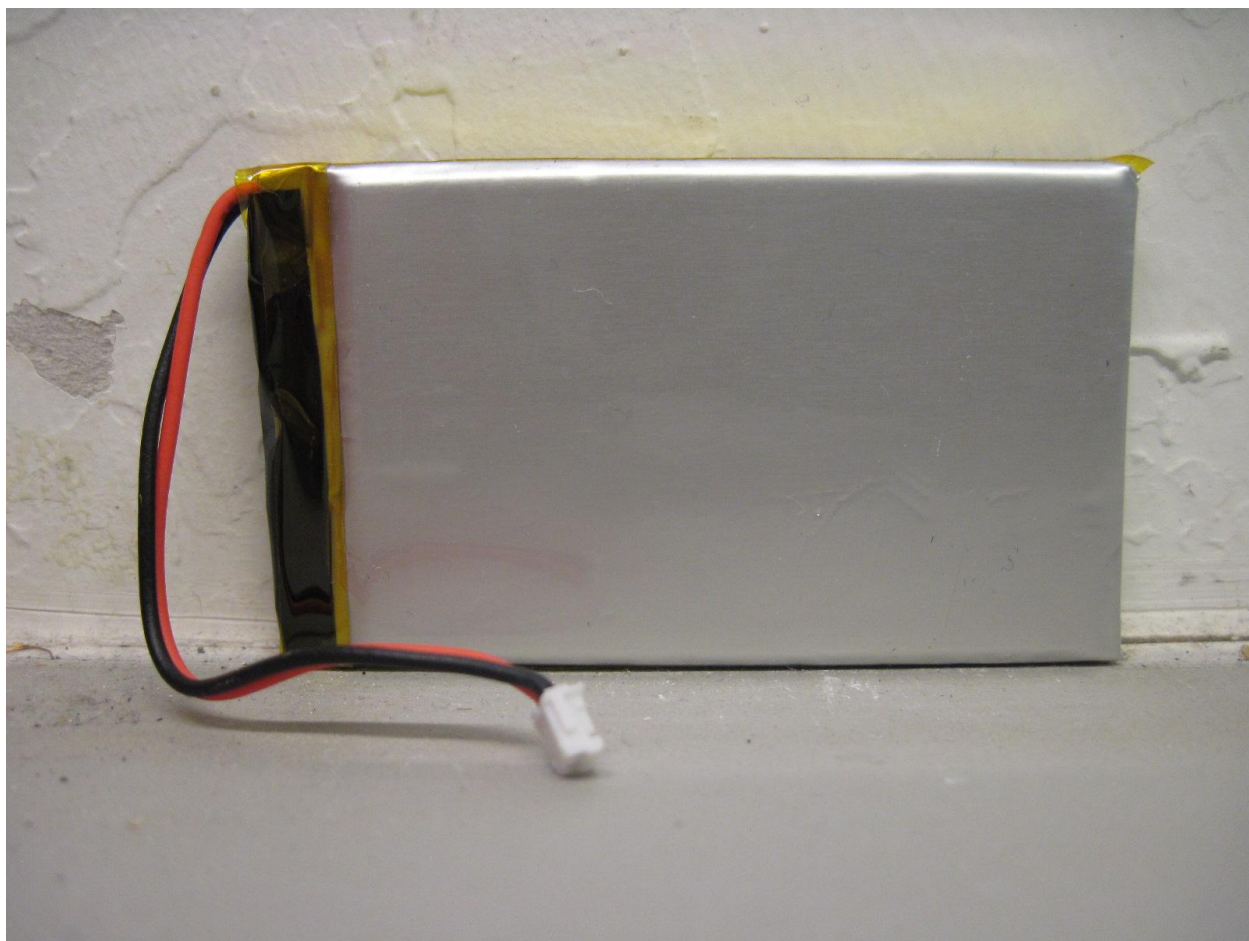
Photograph 1. Battery Back
