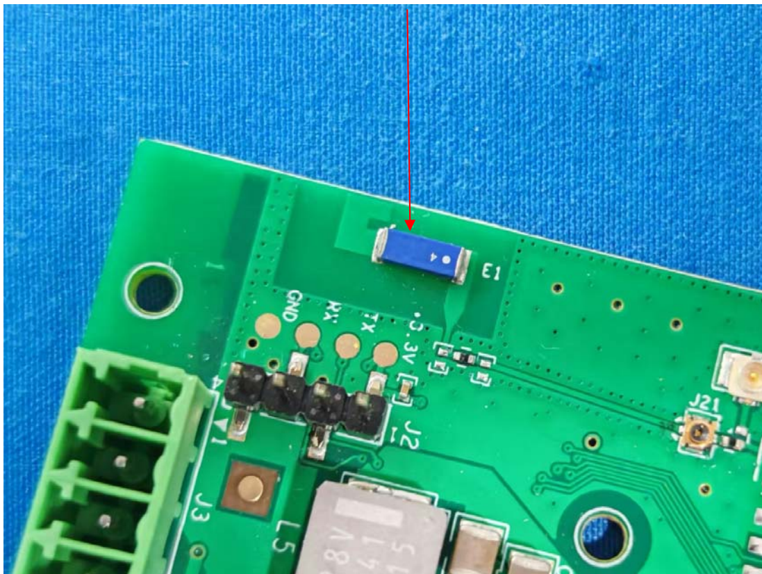
Chip Antenna Chain 0
