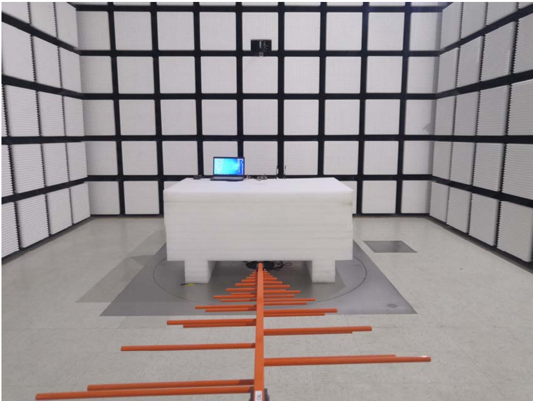
Radiated Emission Below 1GHz Rear View-Whip Antenna
