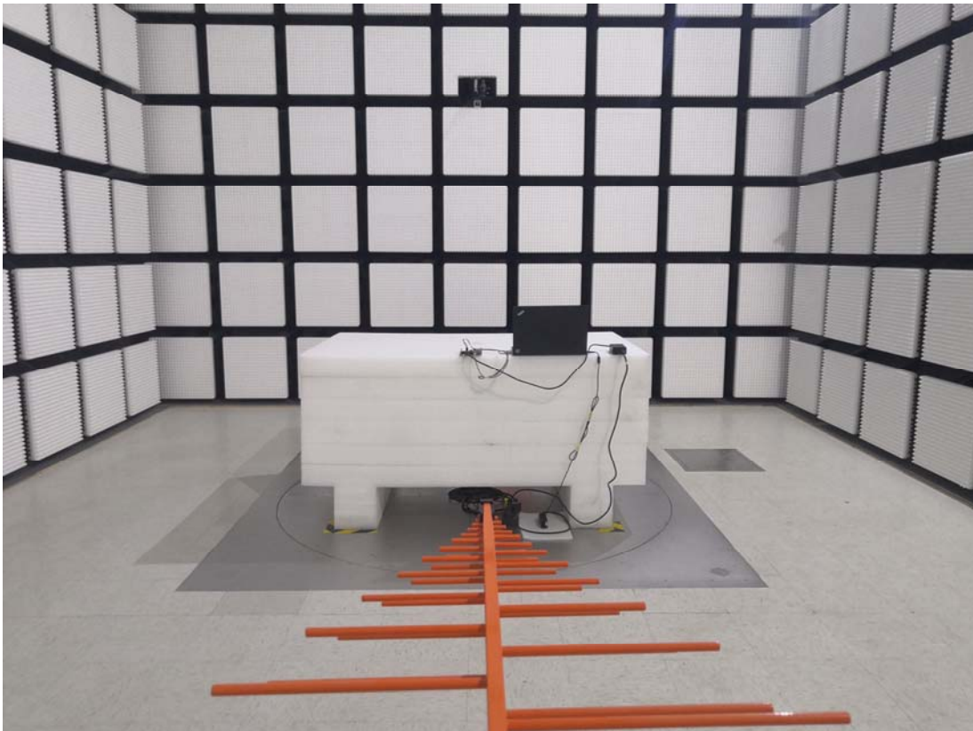
Radiated Emission Below 1GHz Rear View-Chip Antenna
