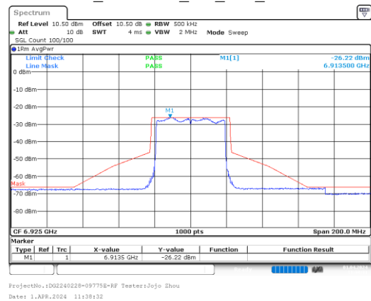
ax40_6925MHz_RU_Full_Chain 1
