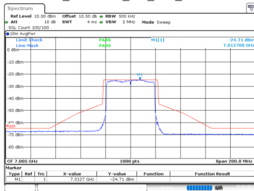
ax40_7005MHz_RU_Full_Chain 2
