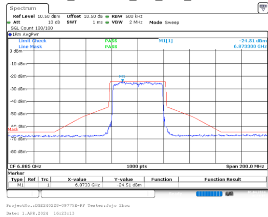
ax40_6885MHz_RU_Full_Chain 3
