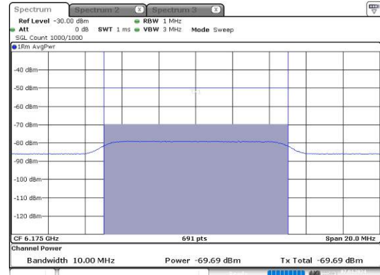
20M-6175-off-2
