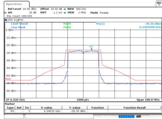
ax20_6535MHz_RU_Full_Chain 3
