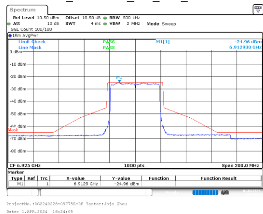
ax40_6925MHz_RU_Full_Chain 3
