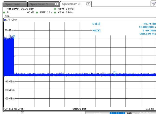
20M-6175-off-1
