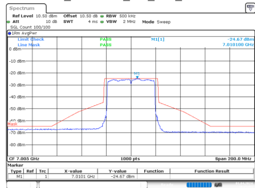
ax40_7005MHz_RU_Full_Chain 3
