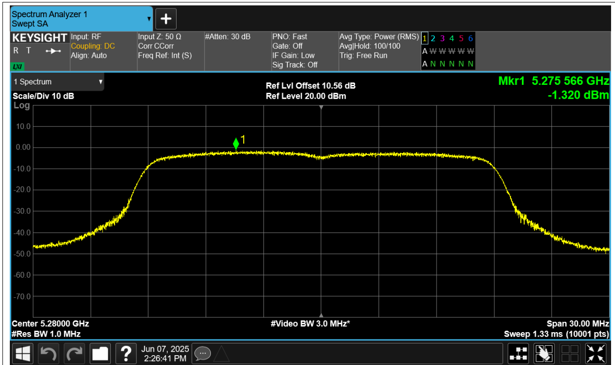
PSD NVNT n20 5280MHz Ant4
