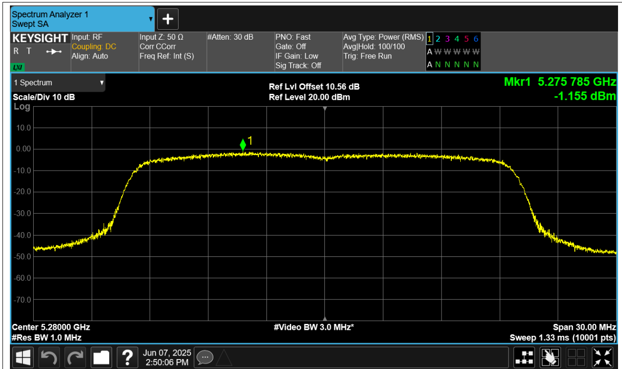
PSD NVNT ax20 5280MHz Ant4
