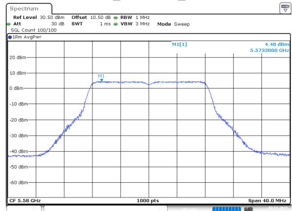
802.11a_5580MHz_Chain 3
