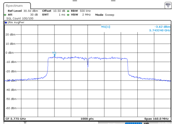
802.11ac80_5775MHz_Chain 3
