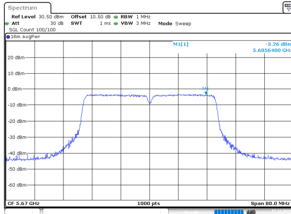
802.11n40_5670MHz_Chain 0
