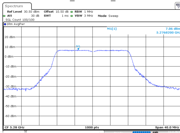
802.11a_5280MHz_Chain 3
