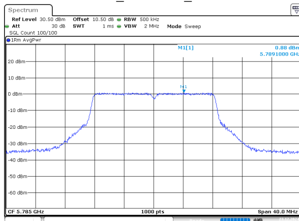
802.11a_5785MHz_Chain 3
