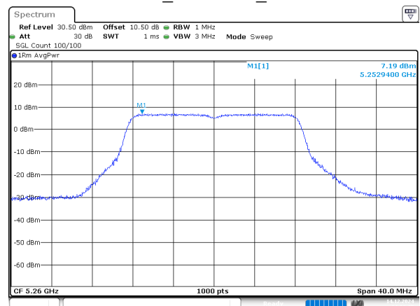
802.11a_5260MHz_Chain 3
