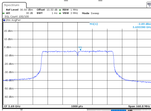
802.11ac80_5690MHz_Chain 2
