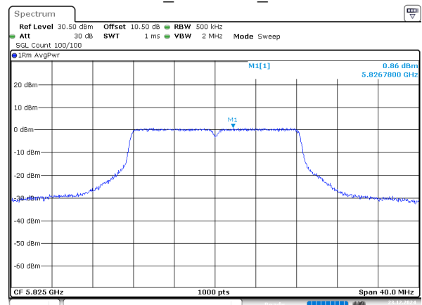
802.11a_5825MHz_Chain 3
