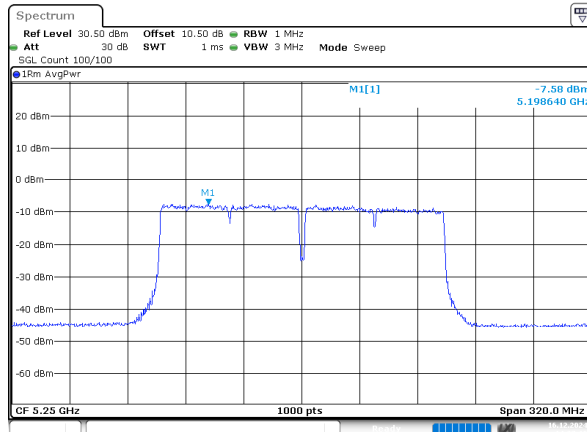
802.11ac160_5250MHz_Chain 0
