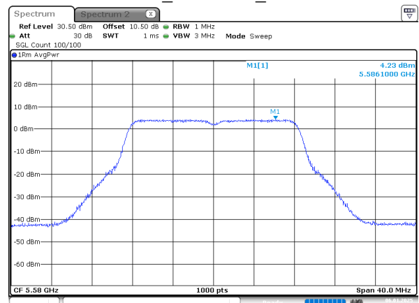
802.11a_5580MHz_Chain 2
