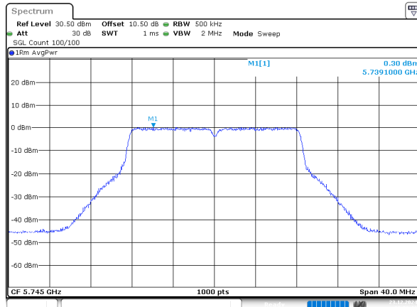
802.11a_5745MHz_Chain 2
