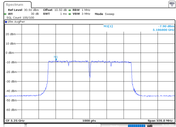
802.11ac160_5250MHz_Chain 1
