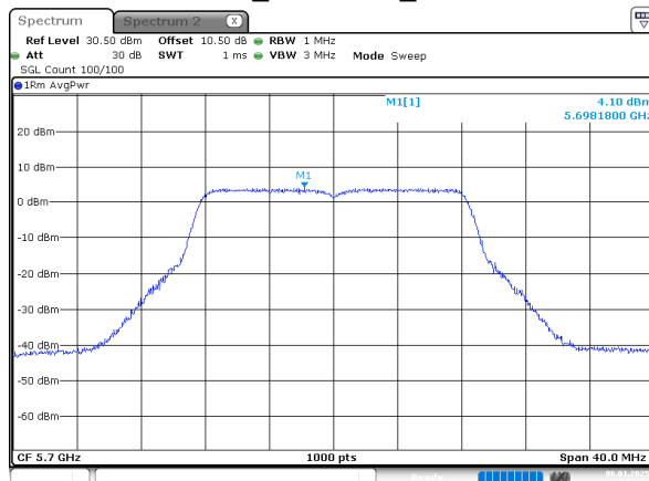
802.11a_5700MHz_Chain 2
