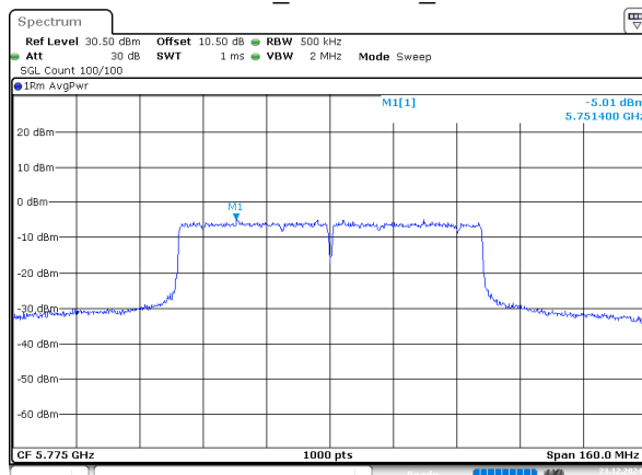
802.11ac80_5775MHz_Chain 2
