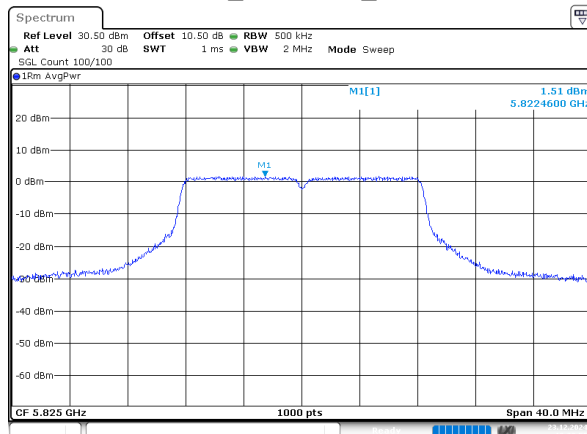
802.11a_5825MHz_Chain 2
