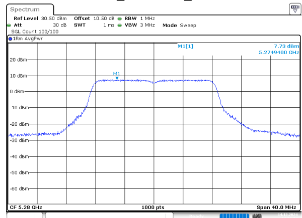
802.11a_5280MHz_Chain 2
