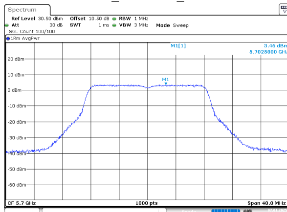
802.11a_5700MHz_Chain 3
