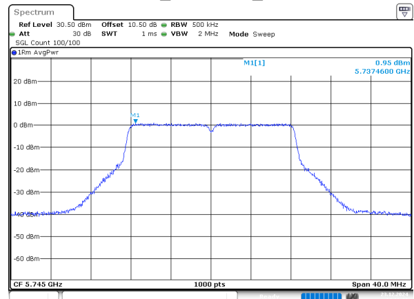
802.11a_5745MHz_Chain 3
