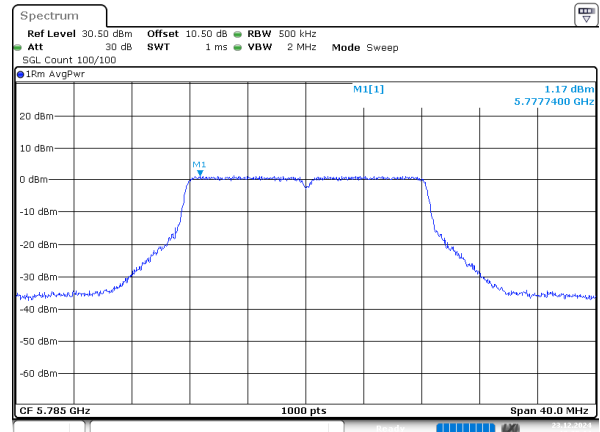
802.11a_5785MHz_Chain 2
