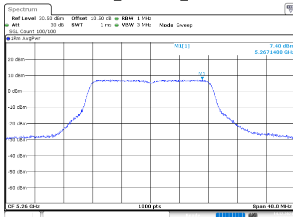
802.11a_5260MHz_Chain 2
