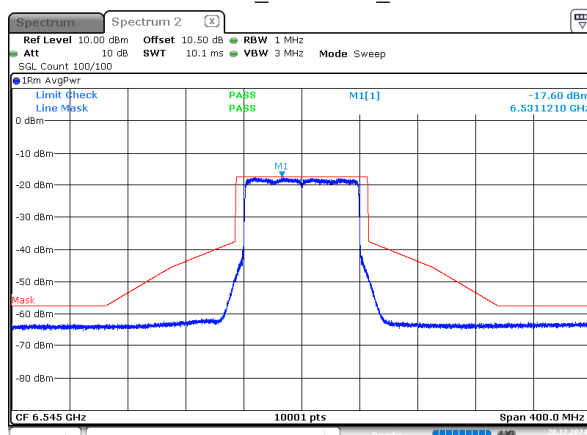
802.11be80 6545MHz Chain 1
