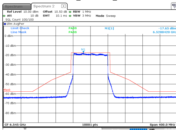
802.11be80 6545MHz Chain 0
