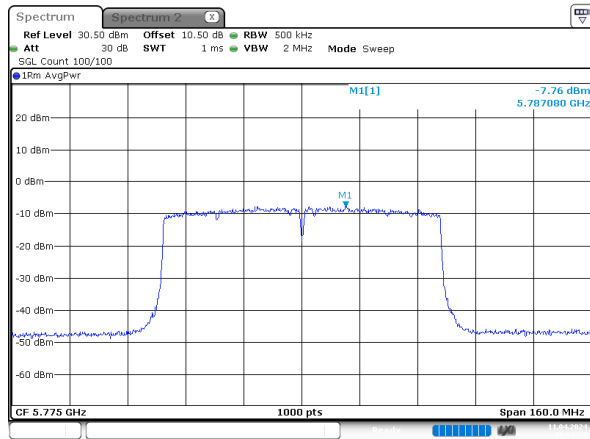
ac80_5775MHz_Chain 0
