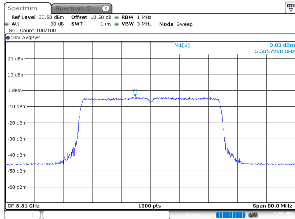
ax40_5510MHz_RU_Full_Chain 0
