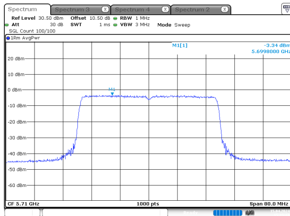
ax40_5710MHz_RU_Full_Chain 2
