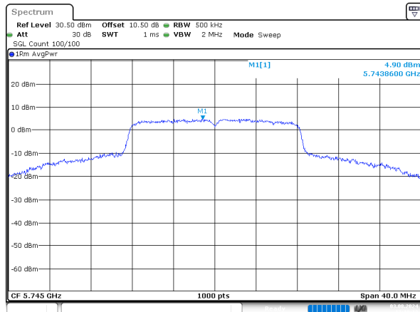
a_5745MHz_Chain 2
