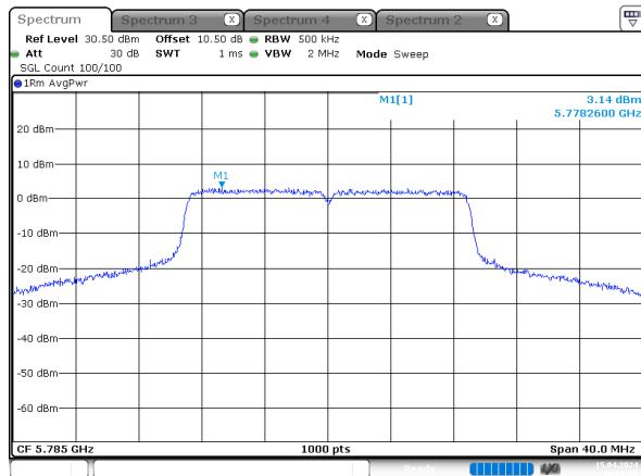
n20_5785MHz_Chain 2
