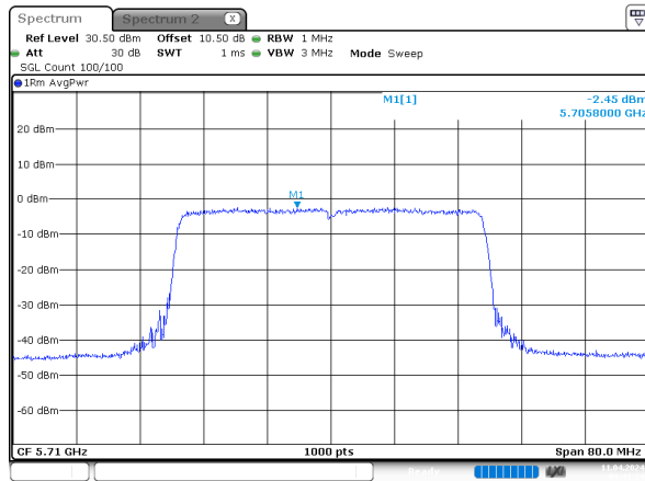
ax40_5710MHz_RU_Full_Chain 0
