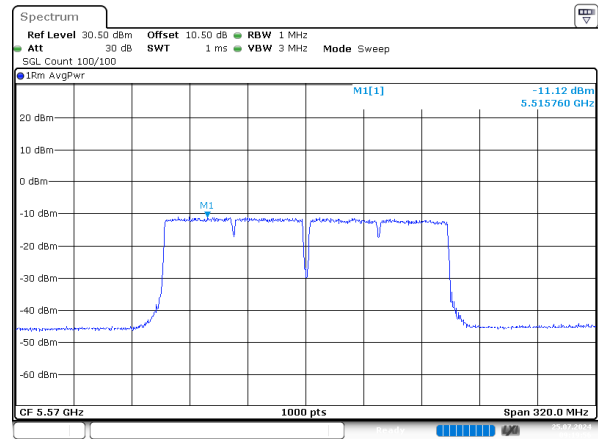
ac160_5570MHz_Chain 1
