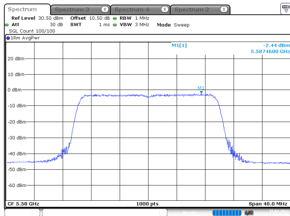
ax20_5580MHz_RU_Full_Chain 2
