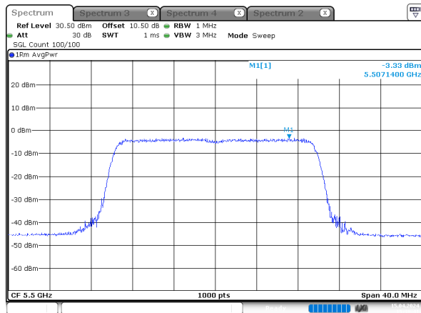
ax20_5500MHz_RU_Full_Chain 2
