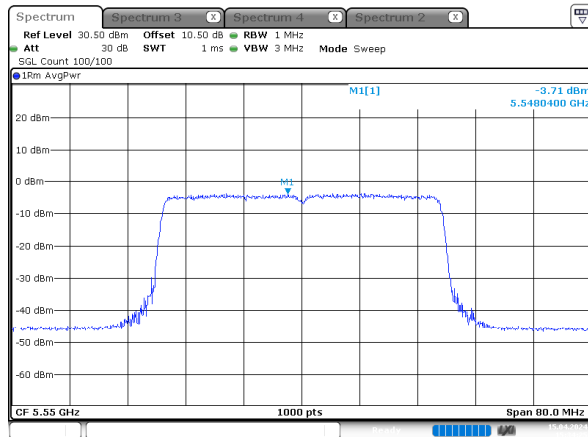
ax40_5550MHz_RU_Full_Chain 2
