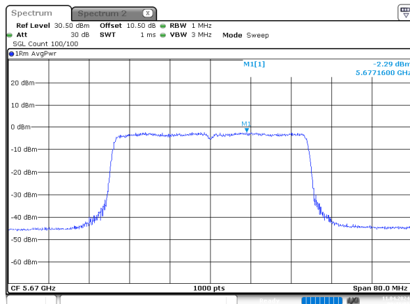
ax40_5670MHz_RU_Full_Chain 0
