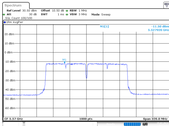
ac160_5570MHz_Chain 2
