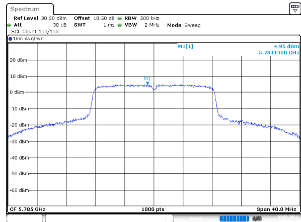
a_5785MHz_Chain 3
