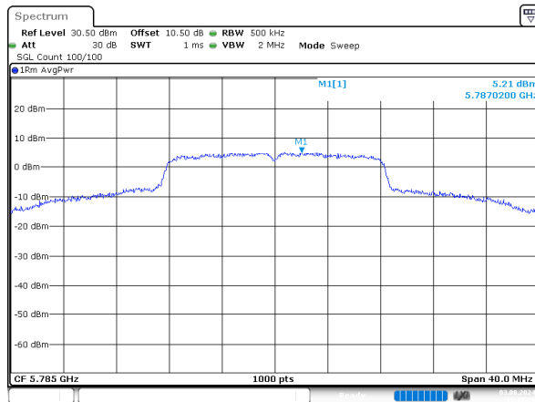
a_5785MHz_Chain 2
