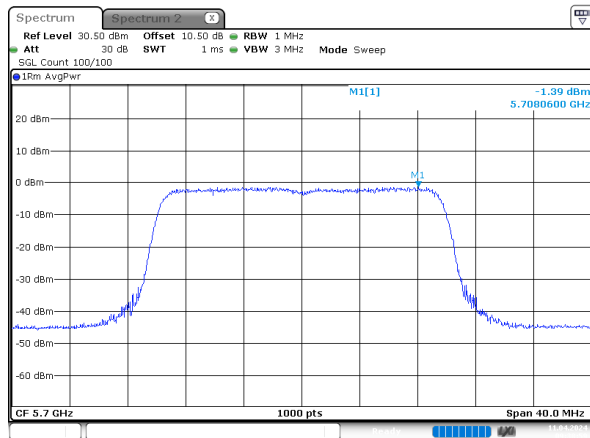
ax20_5700MHz_RU_Full_Chain 0
