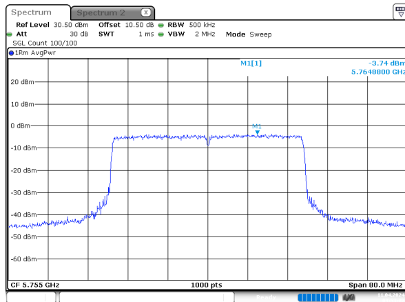
ax40_5755MHz_RU_Full_Chain 0
