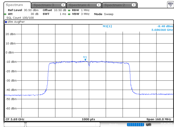
ac80_5690MHz_Chain 1
