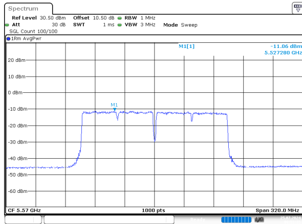
ac160_5570MHz_Chain 0
