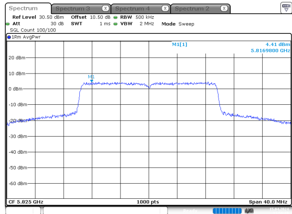
ax20_5825MHz_RU_Full_Chain 1
