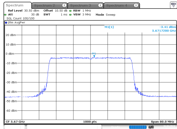
ax40_5670MHz_RU_Full_Chain 3
