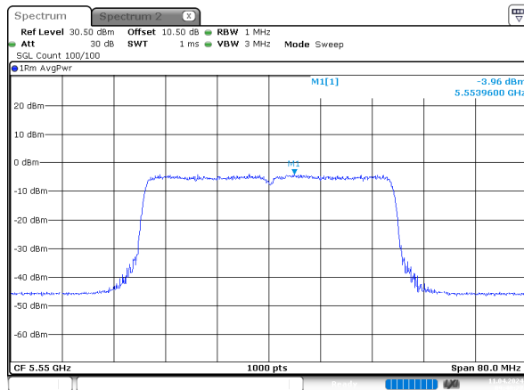
ax40_5550MHz_RU_Full_Chain 0
