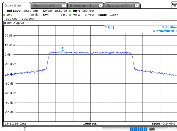
ax20_5785MHz_RU_Full_Chain 2
