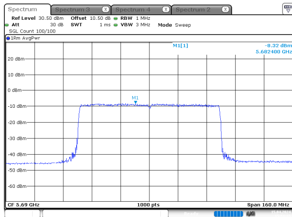
ax80_5690MHz_RU_Full_Chain 2
