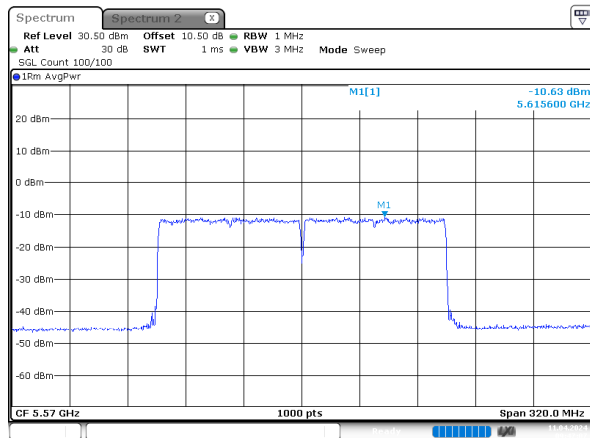
ax160_5570MHz_RU_Full_Chain 0
