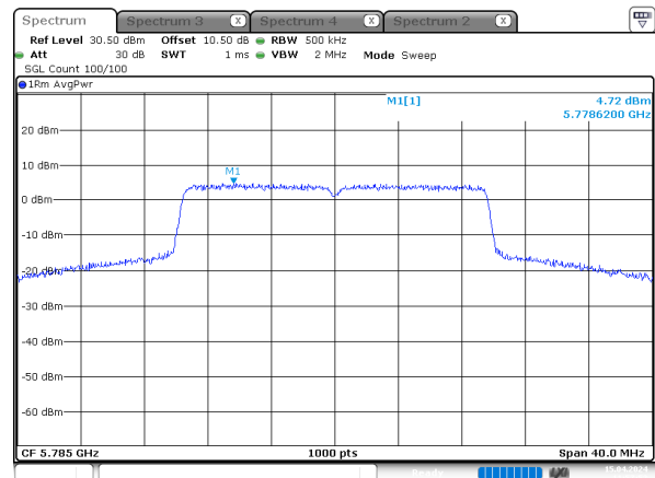
ax20_5785MHz_RU_Full_Chain 1
