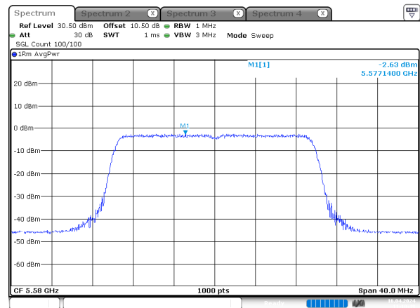
ax20_5580MHz_RU_Full_Chain 3
