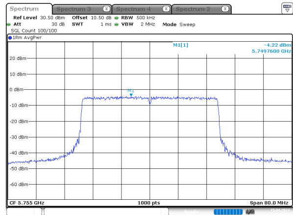
ax40_5755MHz_RU_Full_Chain 1
