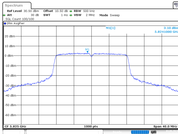
a_5825MHz_Chain 0
