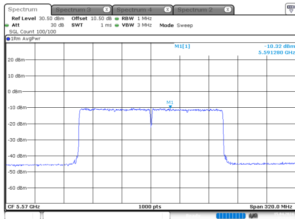
ax160_5570MHz_RU_Full_Chain 2
