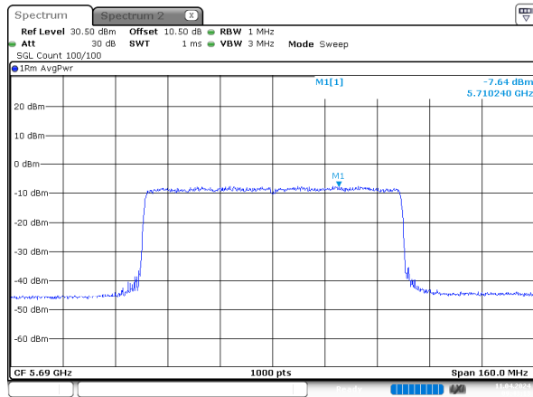
ax80_5690MHz_RU_Full_Chain 0
