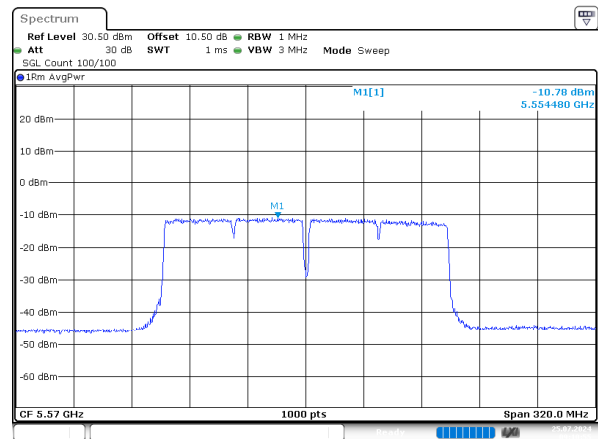
ac160_5570MHz_Chain 3
