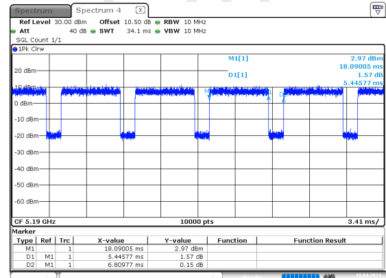
ax40_5190MHz_RU_Full_Chain 0
