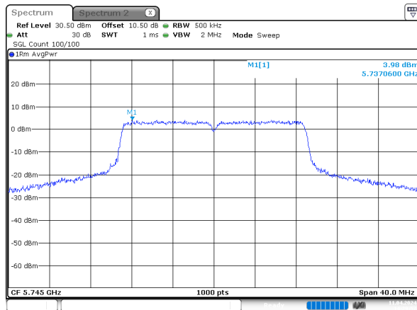
n20_5745MHz_Chain 0
