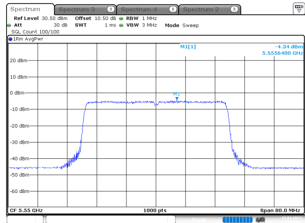
ax40_5550MHz_RU_Full_Chain 1
