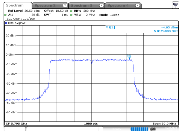
ax40_5795MHz_RU_Full_Chain 3
