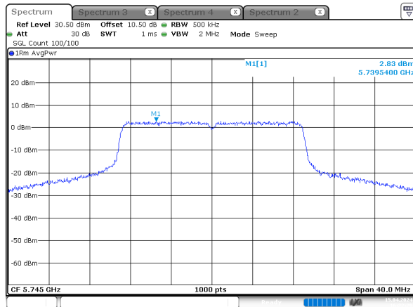
n20_5745MHz_Chain 2
