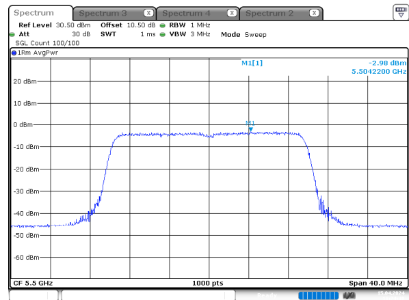
ax20_5500MHz_RU_Full_Chain 1
