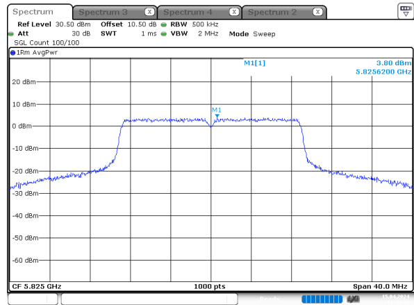
n20_5825MHz_Chain 1
