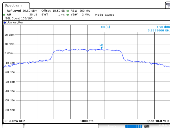
a_5825MHz_Chain 2
