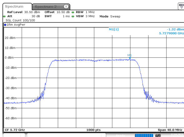
ax20_5720MHz_RU_Full_Chain 0
