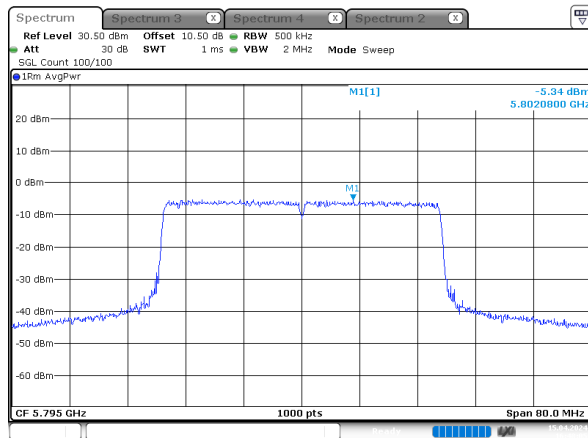
ax40_5795MHz_RU_Full_Chain 2
