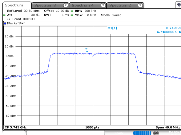
ax20_5745MHz_RU_Full_Chain 2
