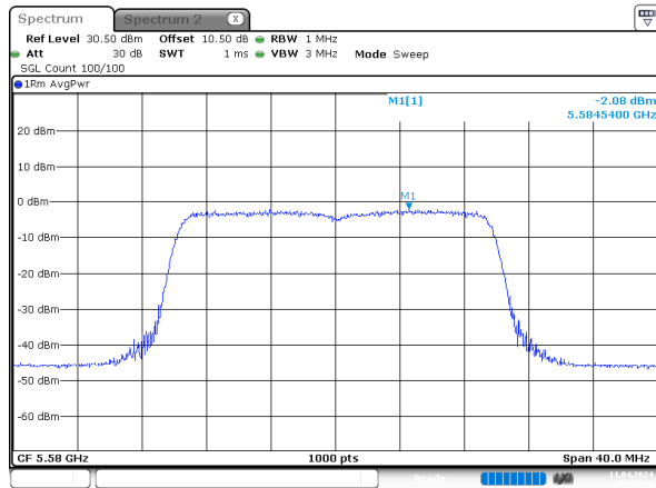
ax20_5580MHz_RU_Full_Chain 0
