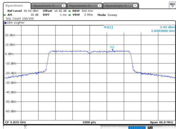
ax20_5825MHz_RU_Full_Chain 3
