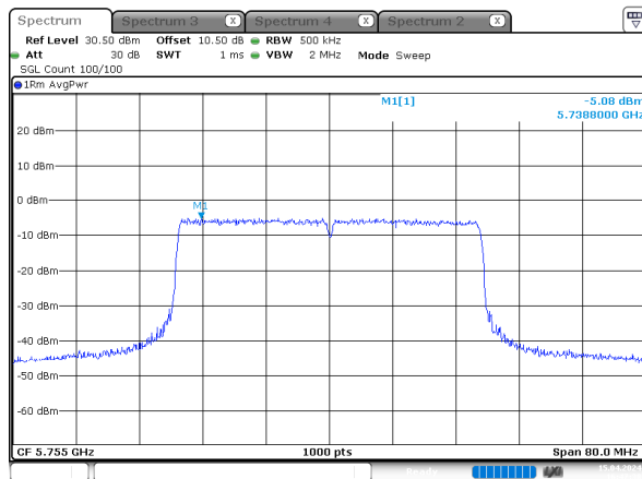
ax40_5755MHz_RU_Full_Chain 2
