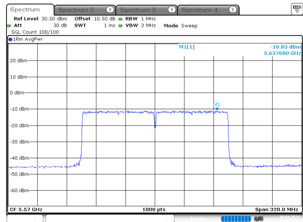
ax160_5570MHz_RU_Full_Chain 3
