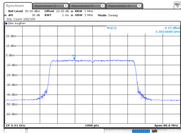
ax40_5510MHz_RU_Full_Chain 3
