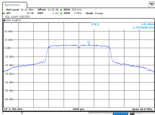
a_5785MHz_Chain 1
