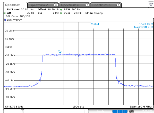
ax80_5775MHz_RU_Full_Chain 3
