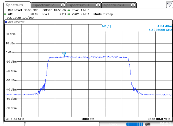
ax40_5550MHz_RU_Full_Chain 3
