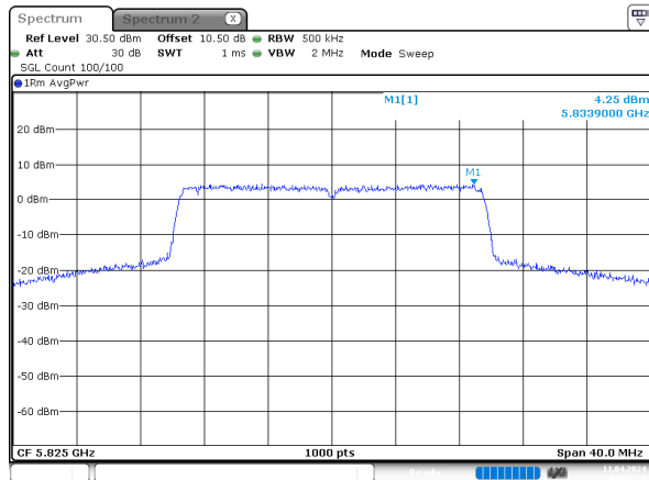
ax20_5825MHz_RU_Full_Chain 0
