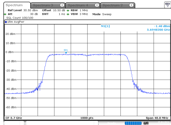
ax20_5700MHz_RU_Full_Chain 1
