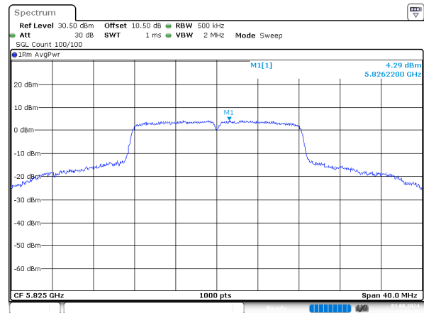
a_5825MHz_Chain 1
