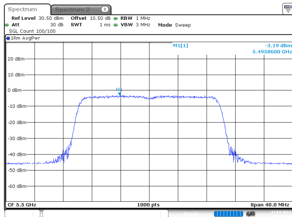
ax20_5500MHz_RU_Full_Chain 0
