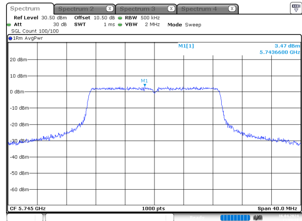
n20_5745MHz_Chain 3
