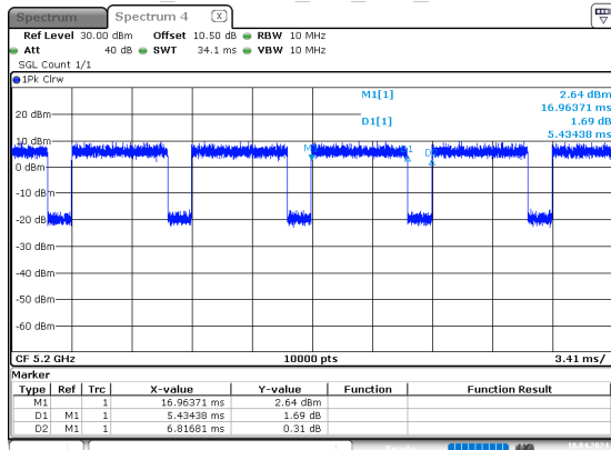
ax20_5200MHz_RU_Full_Chain 0
