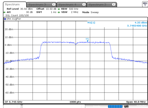
ax20_5745MHz_RU_Full_Chain 1
