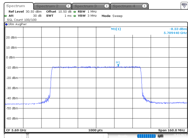
ax80_5690MHz_RU_Full_Chain 3
