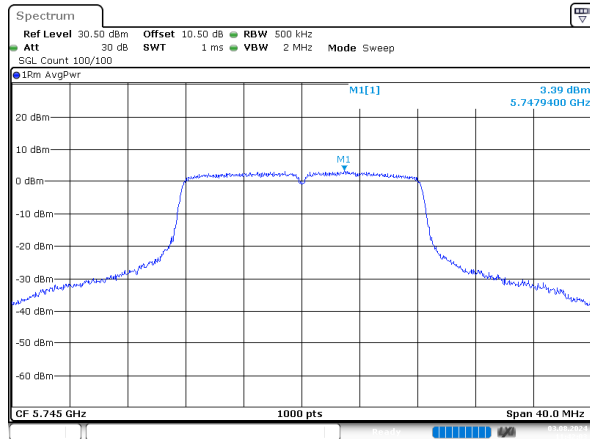
a_5745MHz_Chain 0
