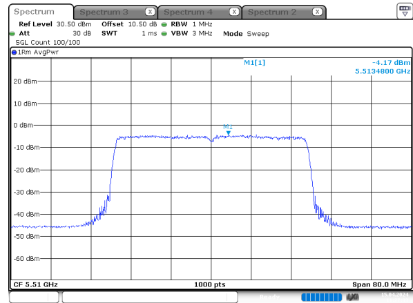
ax40_5510MHz_RU_Full_Chain 1
