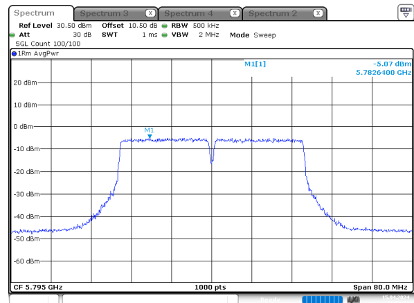
n40_5795MHz_Chain 1
