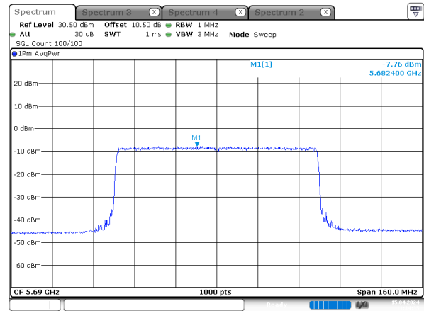
ax80_5690MHz_RU_Full_Chain 1
