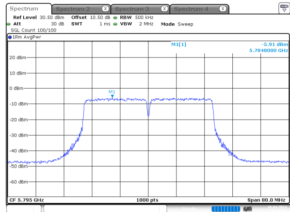
n40_5795MHz_Chain 3
