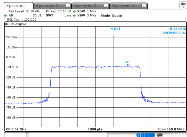
ax80_5610MHz_RU_Full_Chain 3
