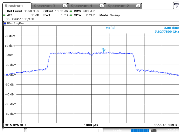
ax20_5825MHz_RU_Full_Chain 2
