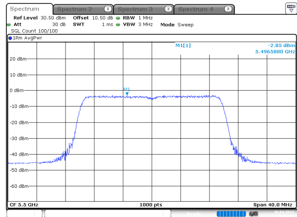
ax20_5500MHz_RU_Full_Chain 3
