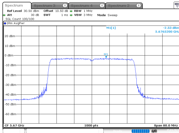
ax40_5670MHz_RU_Full_Chain 2
