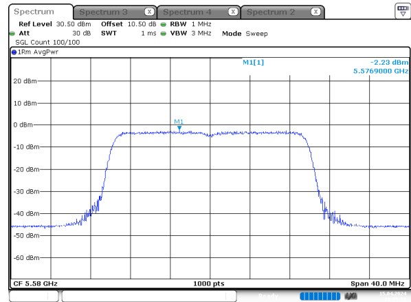
ax20_5580MHz_RU_Full_Chain 1
