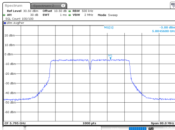
n40_5795MHz_Chain 0
