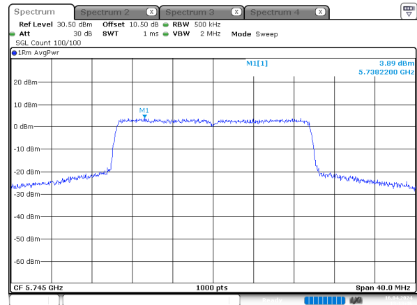
ax20_5745MHz_RU_Full_Chain 3
