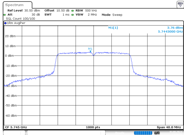
a_5745MHz_Chain 1
