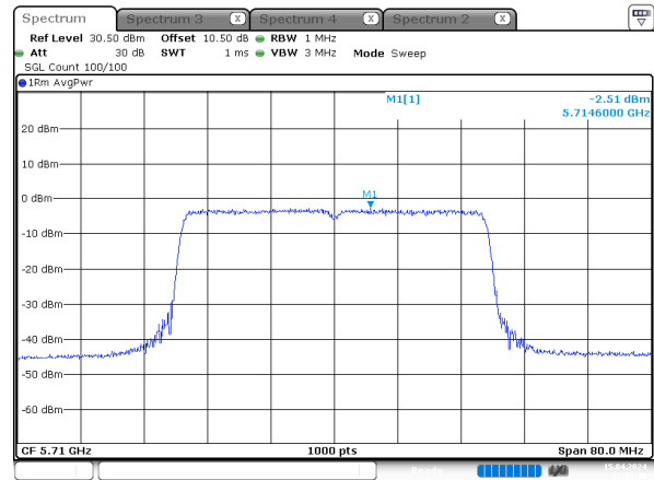
ax40_5710MHz_RU_Full_Chain 1
