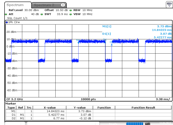
n20_5200MHz_Chain 0
