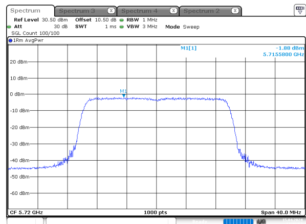
ax20_5720MHz_RU_Full_Chain 1
