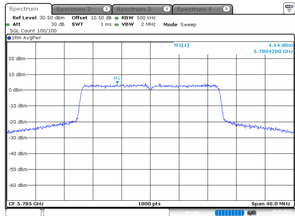
ax20_5785MHz_RU_Full_Chain 3
