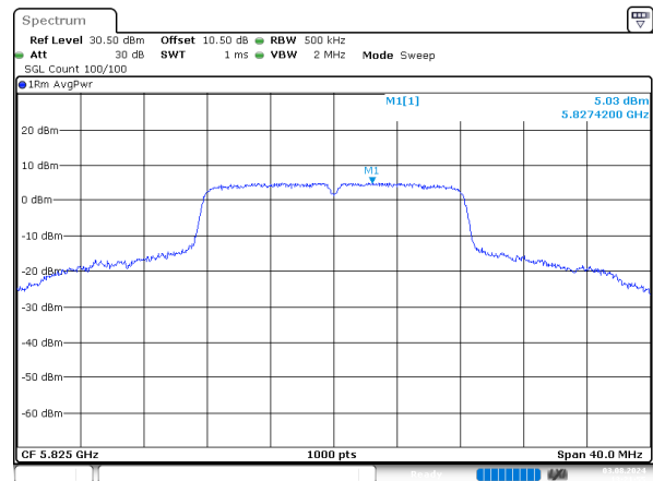
a_5825MHz_Chain 3
