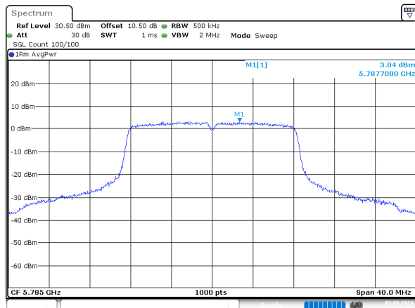
a_5785MHz_Chain 0
