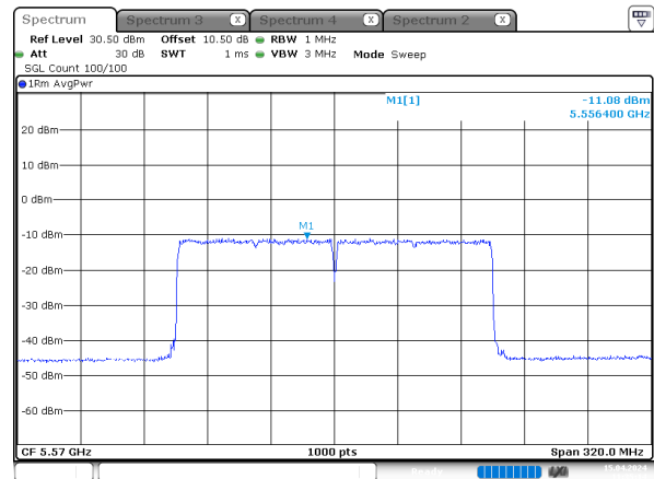
ax160_5570MHz_RU_Full_Chain 1
