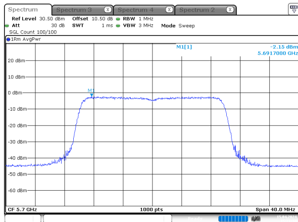
ax20_5700MHz_RU_Full_Chain 2
