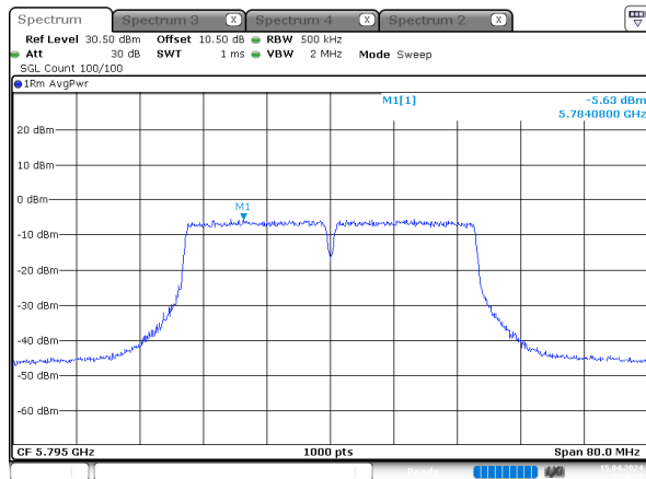
n40_5795MHz_Chain 2
