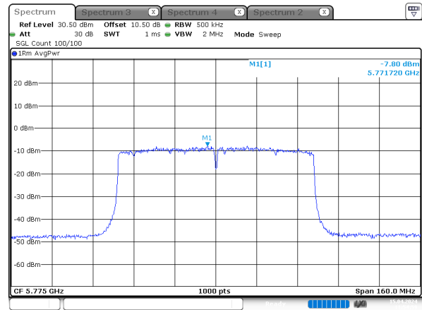
ac80_5775MHz_Chain 1
