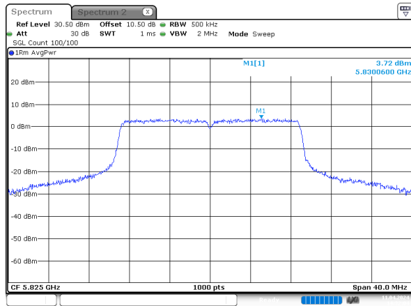
n20_5825MHz_Chain 0
