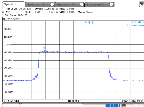
ax80_5610MHz_RU_Full_Chain 2
