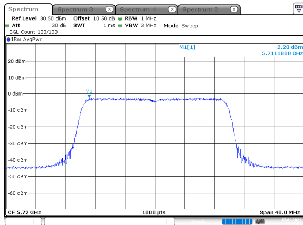
ax20_5720MHz_RU_Full_Chain 2
