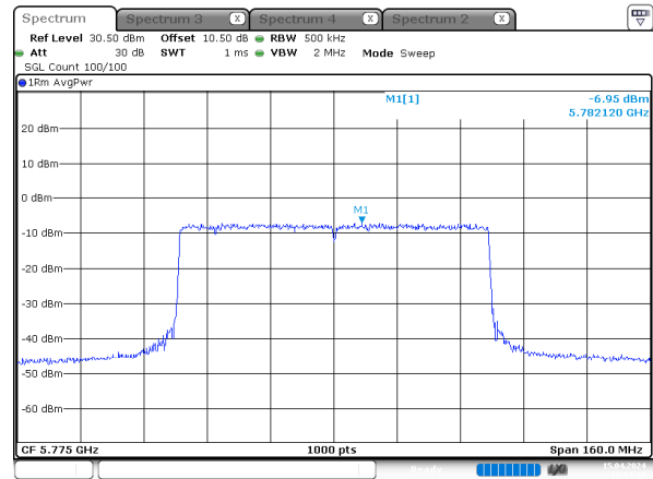
ax80_5775MHz_RU_Full_Chain 1
