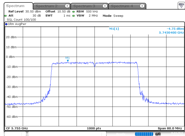
ax40_5755MHz_RU_Full_Chain 3
