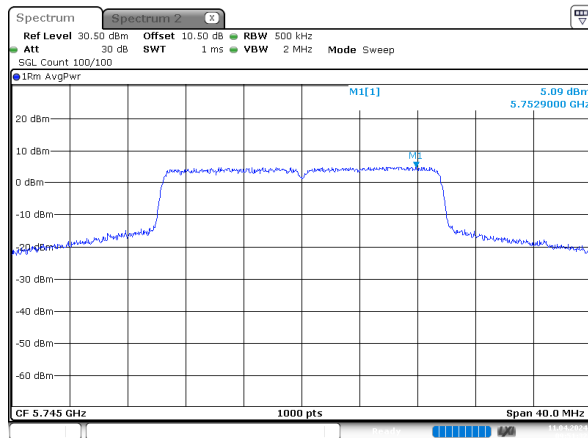
ax20_5745MHz_RU_Full_Chain 0 z
