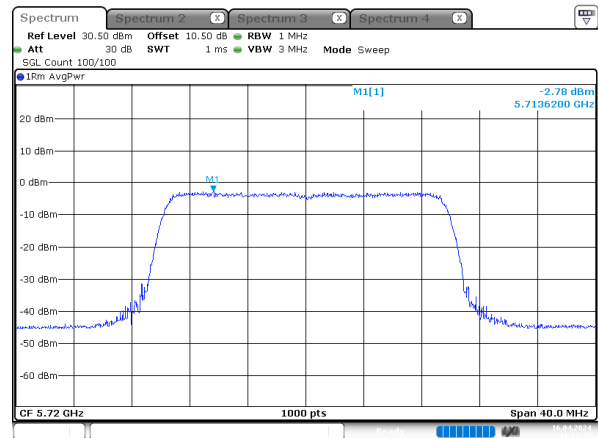
ax20_5720MHz_RU_Full_Chain 3
