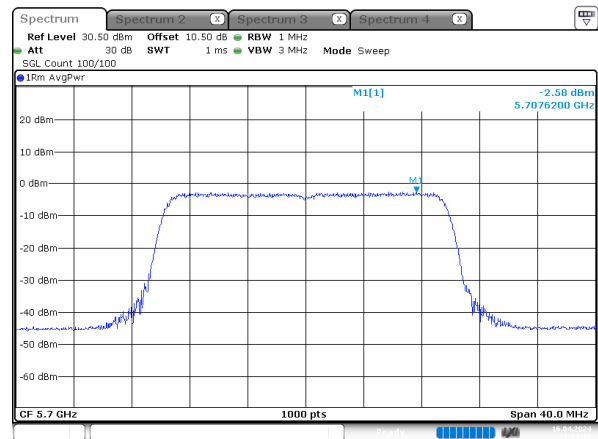
ax20_5700MHz_RU_Full_Chain 3
