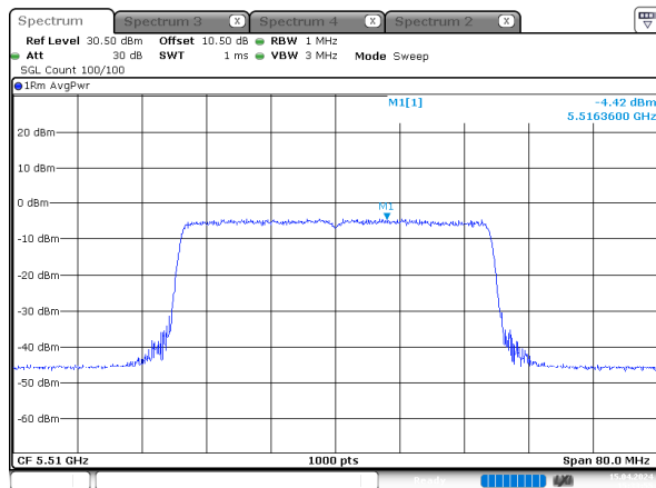
ax40_5510MHz_RU_Full_Chain 2
