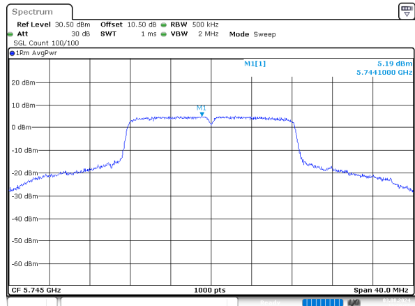
a_5745MHz_Chain 3
