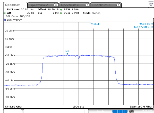
ac80_5690MHz_Chain 3
