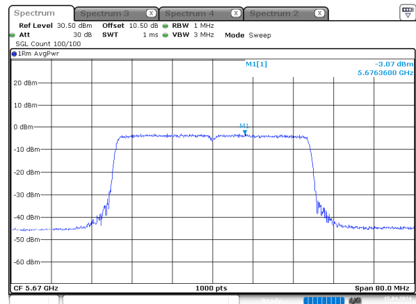
ax40_5670MHz_RU_Full_Chain 1
