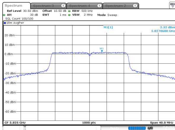
n20_5825MHz_Chain 2
