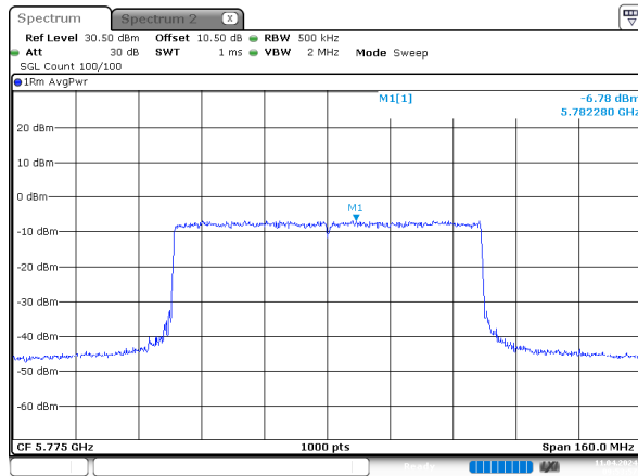
ax80_5775MHz_RU_Full_Chain 0
