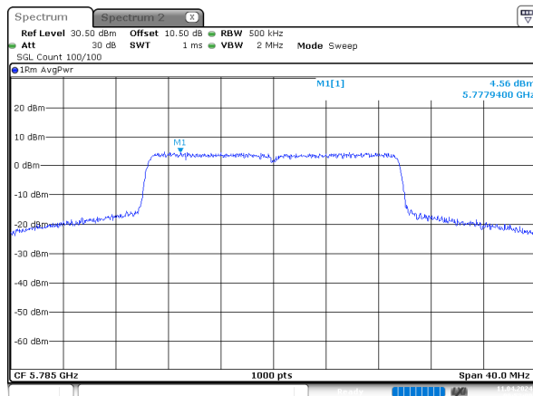
ax20_5785MHz_RU_Full_Chain 0
