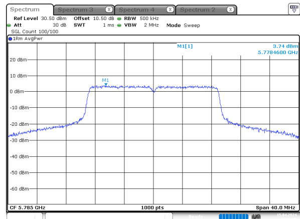
n20_5785MHz_Chain 1
