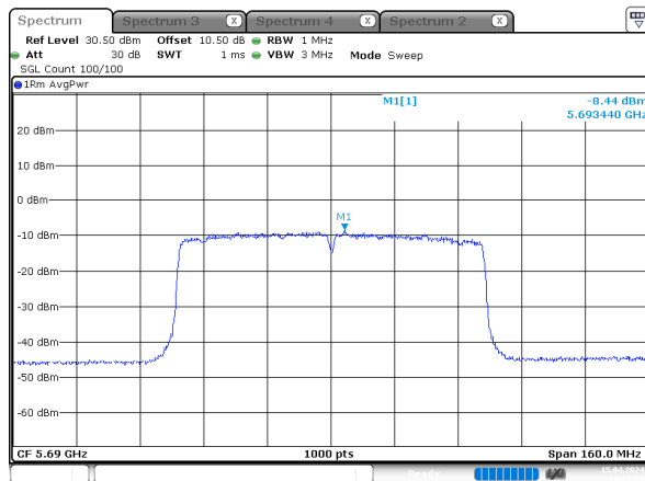
ac80_5690MHz_Chain 2
