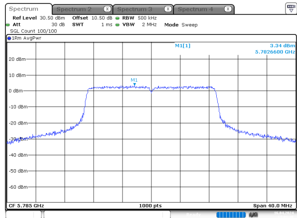
n20_5785MHz_Chain 3
