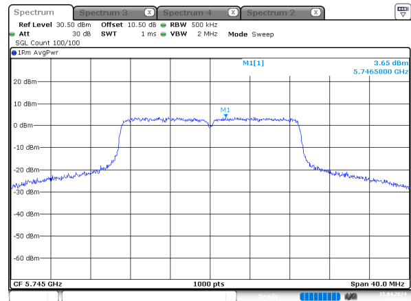
n20_5745MHz_Chain 1
