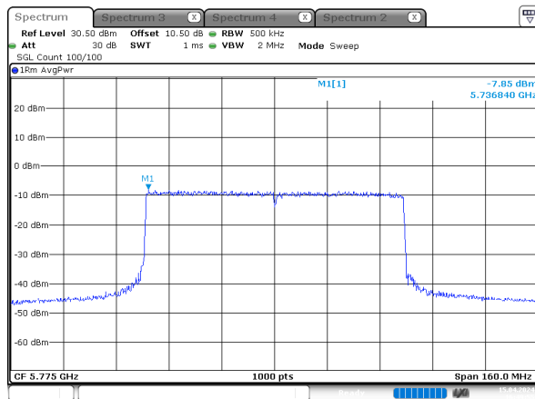
ax80_5775MHz_RU_Full_Chain 2
