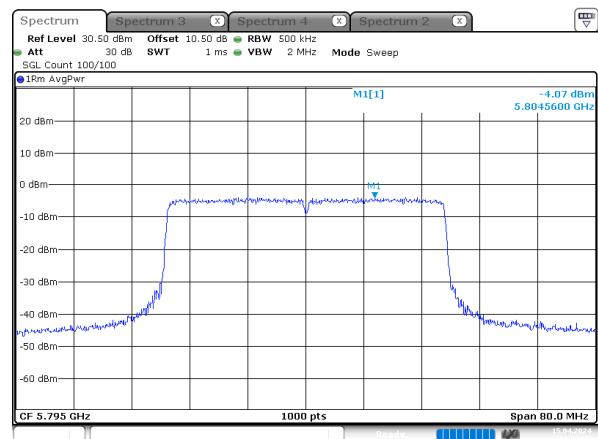
ax40_5795MHz_RU_Full_Chain 1
