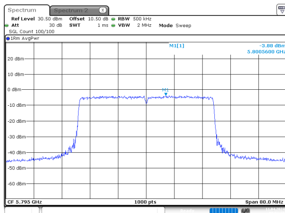
ax40_5795MHz_RU_Full_Chain 0
