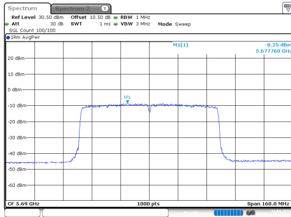
ac80_5690MHz_Chain 0
