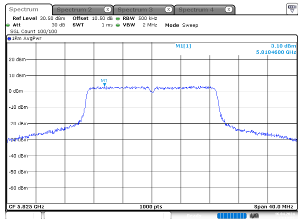
n20_5825MHz_Chain 3
