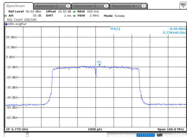
ac80_5775MHz_Chain 3
