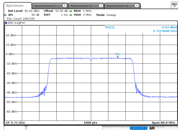
ax40_5710MHz_RU_Full_Chain 3
