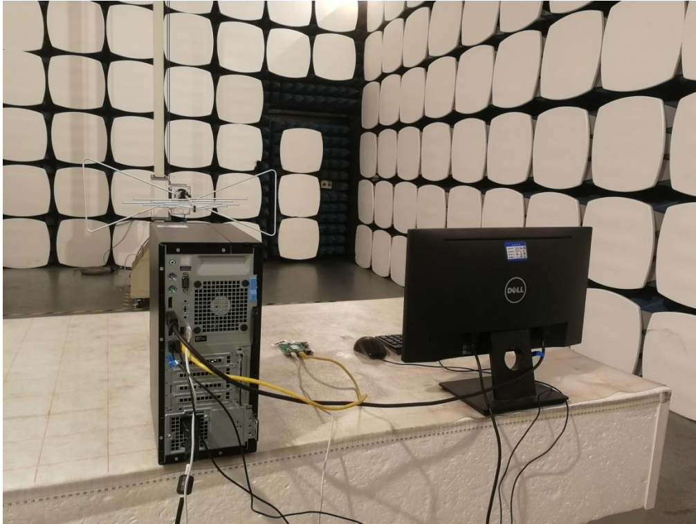
Radiated Spurious Emission (Flex Antenna) Below 1GHz
