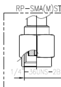
Detail B Scale:5:1
