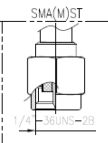
Detail C Scale:5:1
