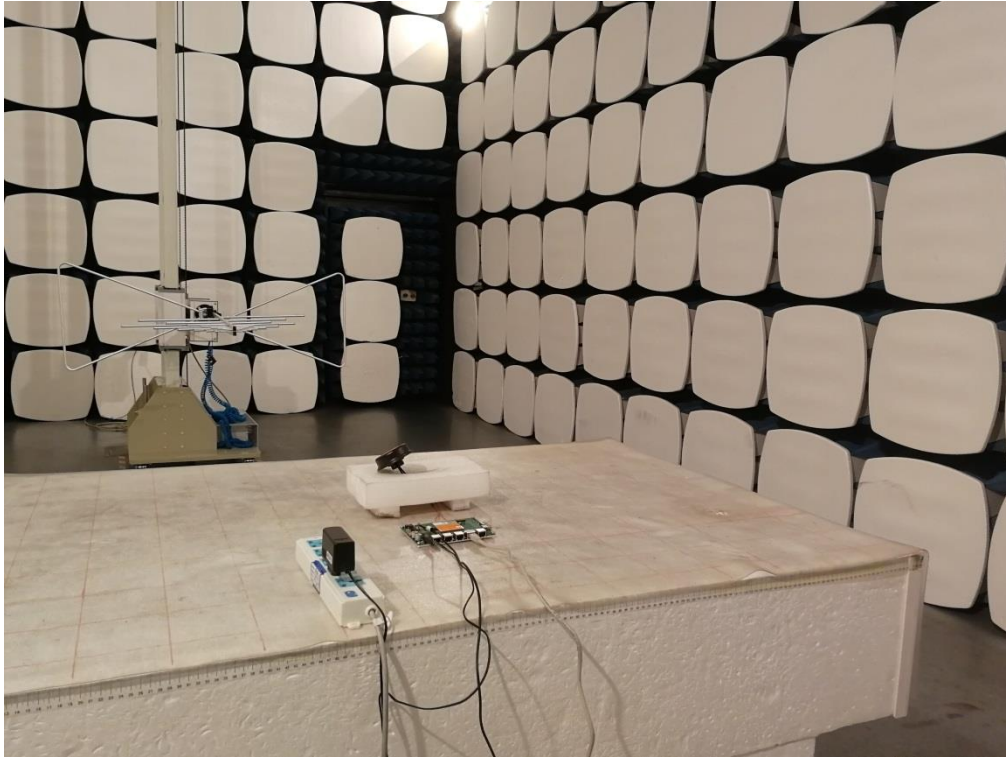
Radiated Spurious Emission (Planare WLAN Antenne) Below 1GHz
