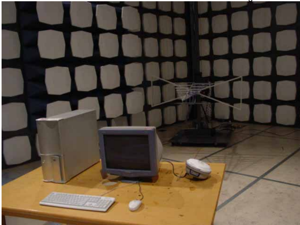
FCC RADIATED EMISSION TEST SETUP-Reading
