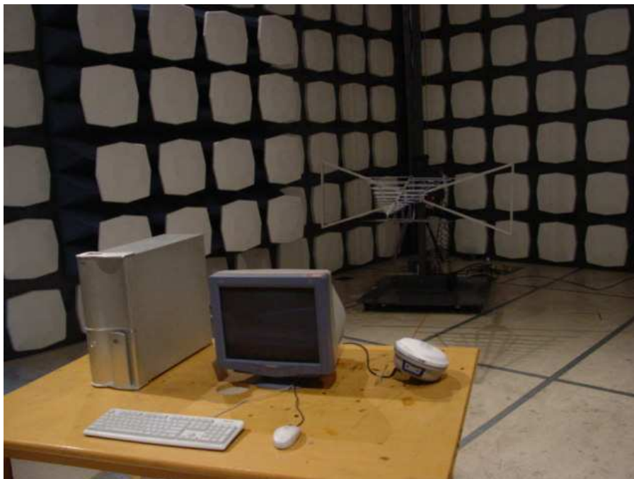
FCC RADIATED EMISSION TEST SETUP-Reading
