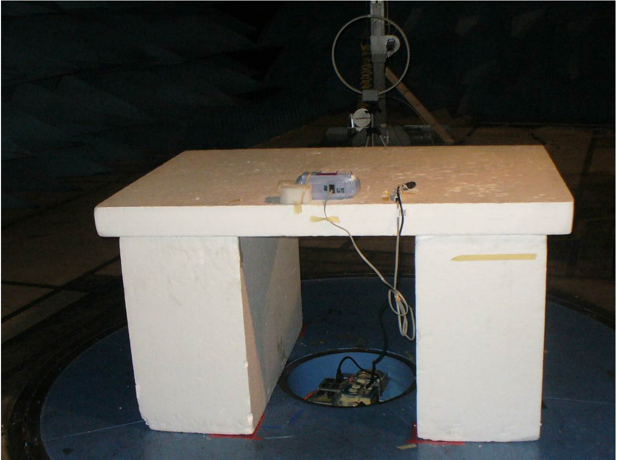
Figure 2: Radiated Emissions – Back View – FCC 15.209
