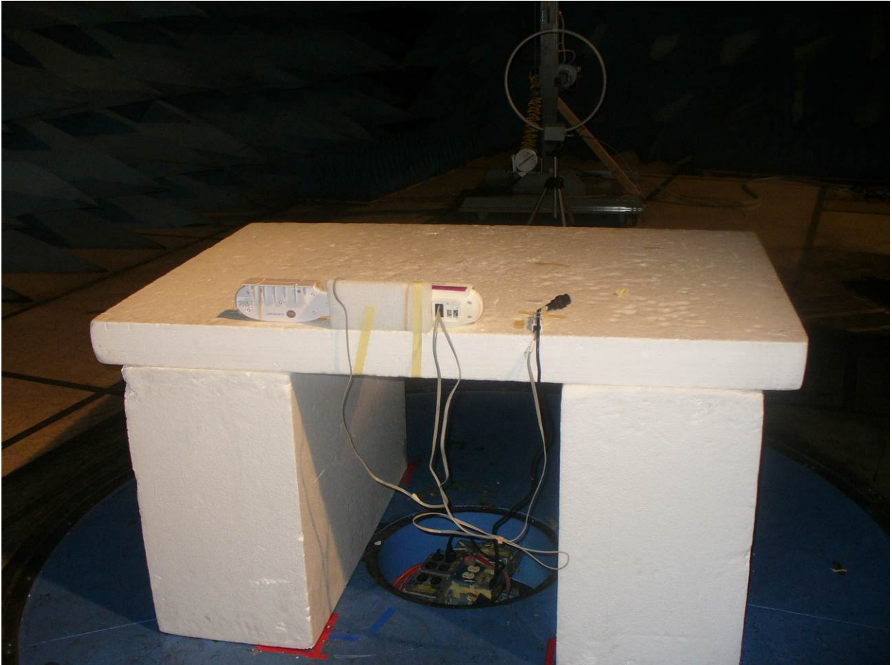
Figure 5: Radiated Emissions – Back View – FCC 15.209, 15.231, 15.249
