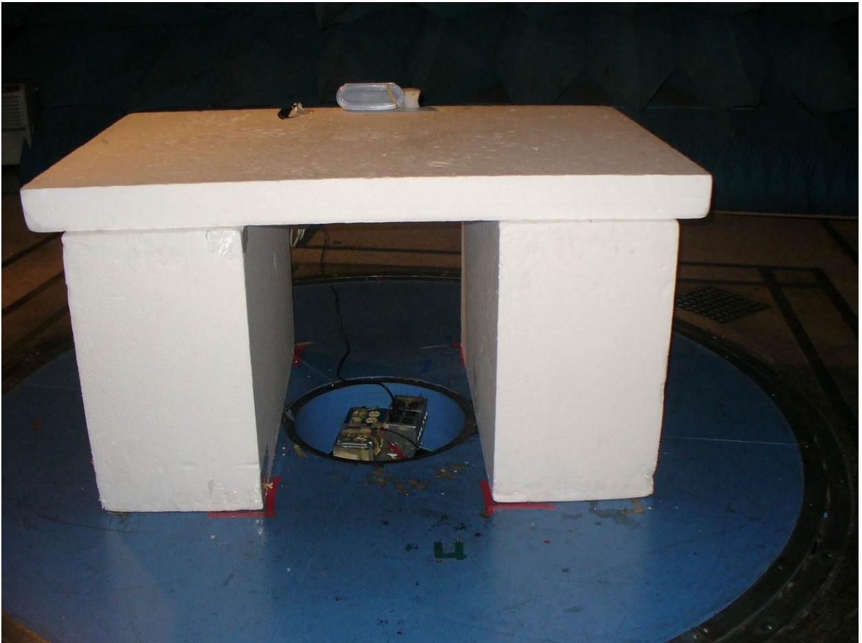
Figure 1: Radiated Emissions – Front View – FCC 15.209
