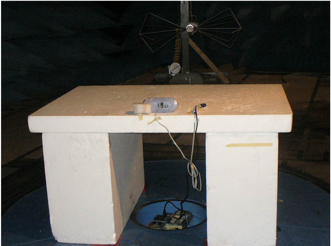
Figure 3: Radiated Emissions – Back View – FCC 15.209
