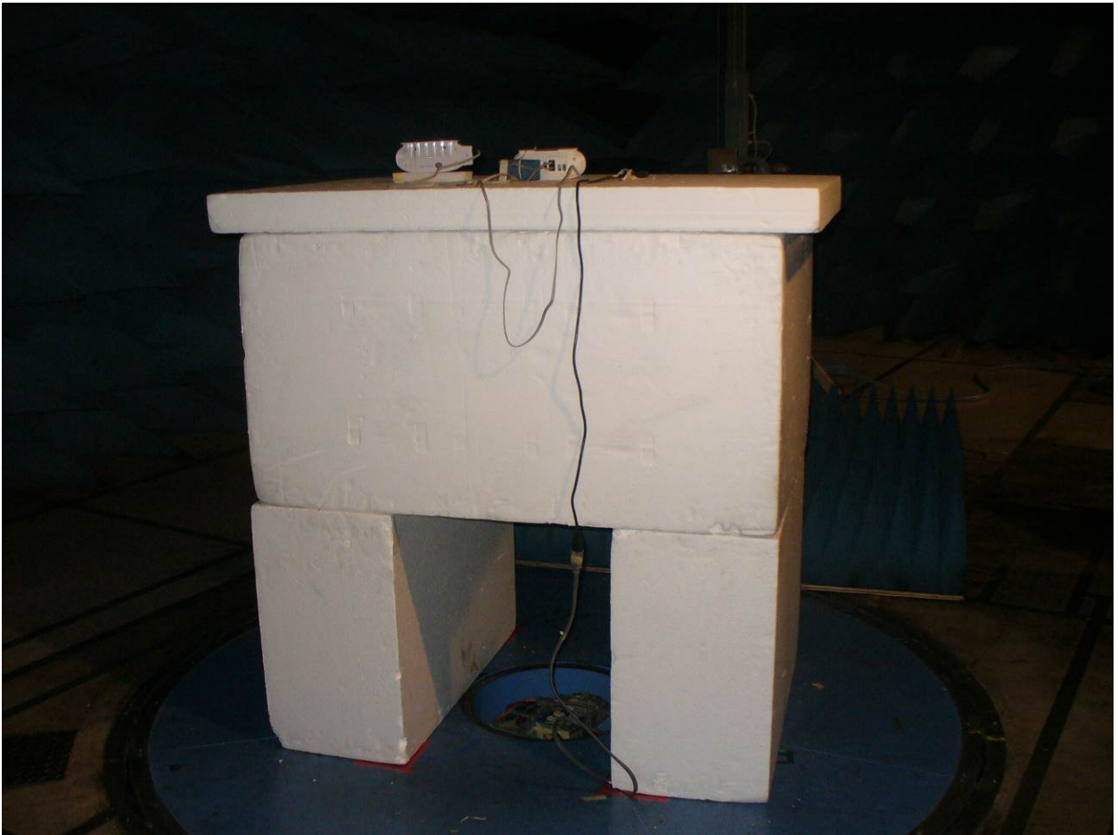
Figure 9: Radiated Emissions – Back View – FCC 15.231, 15.249
