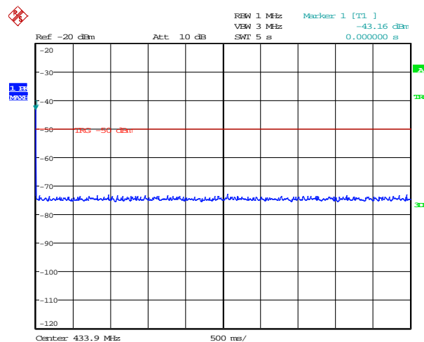
Figure 7.4.2-1: Periodic Operation
