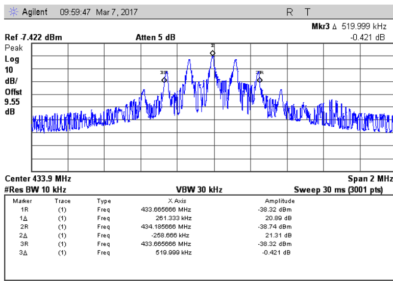
Figure 7.2.2-1: 20dB BW
