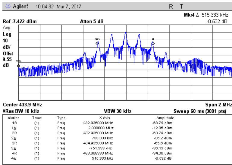
Figure 7.2.2-2: 99% OBW
