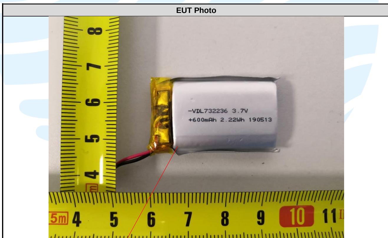
Battery 2: VDL732236
