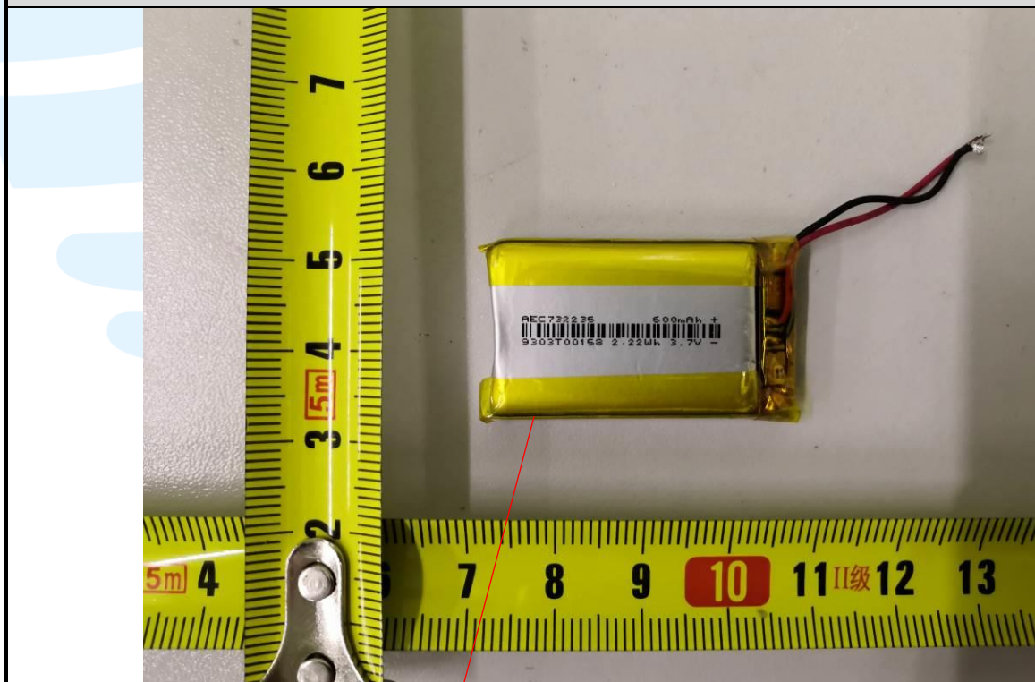
Battery 1 AEC732236
