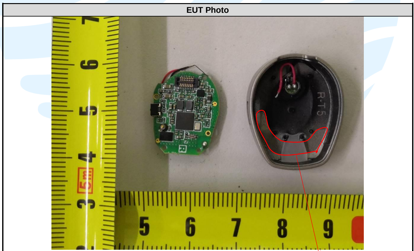
BT Antenna
