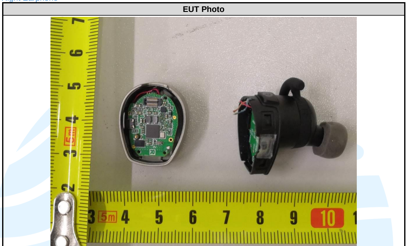
Right Earphone
