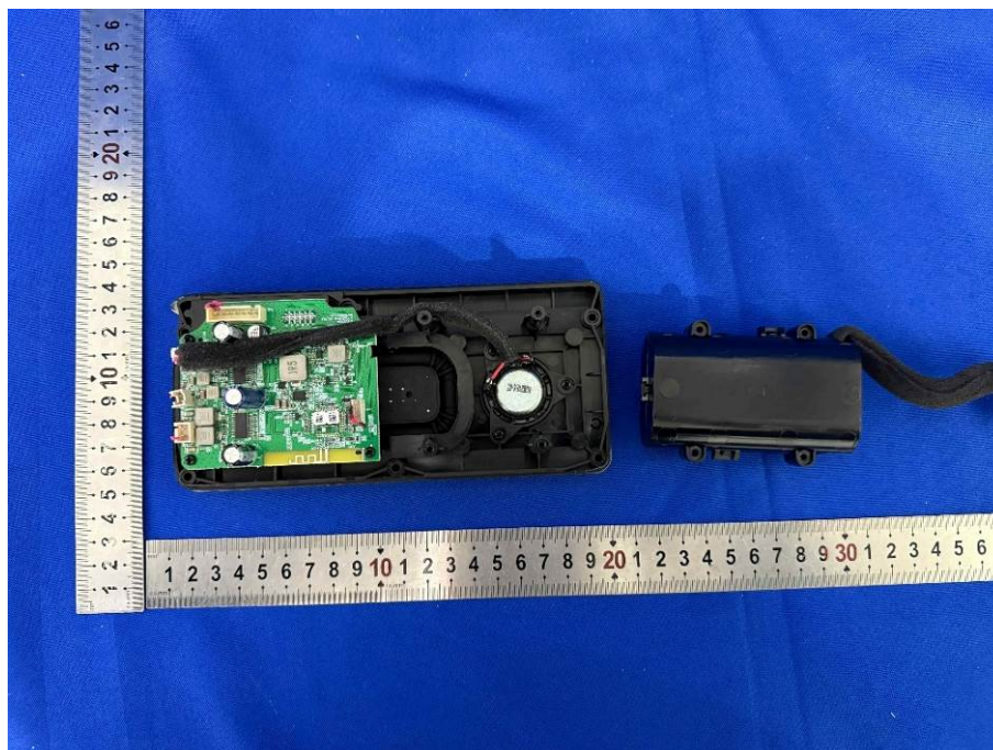
Figure 9: Internal view_4
