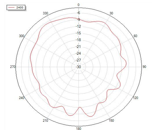
Phi=90 freq=2400MHz
