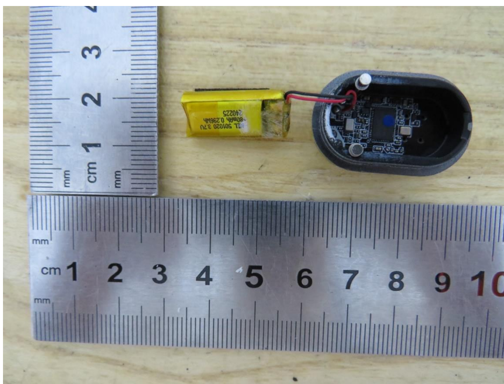
Internal View of EUT-8-R
