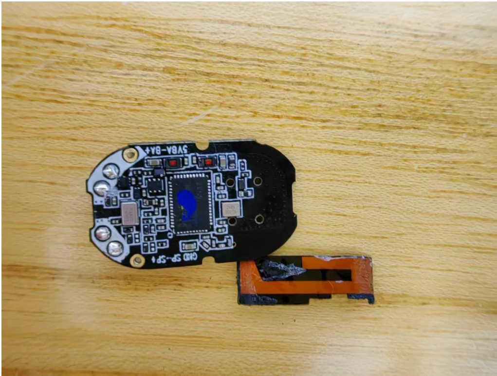
Internal View of EUT-6-L
