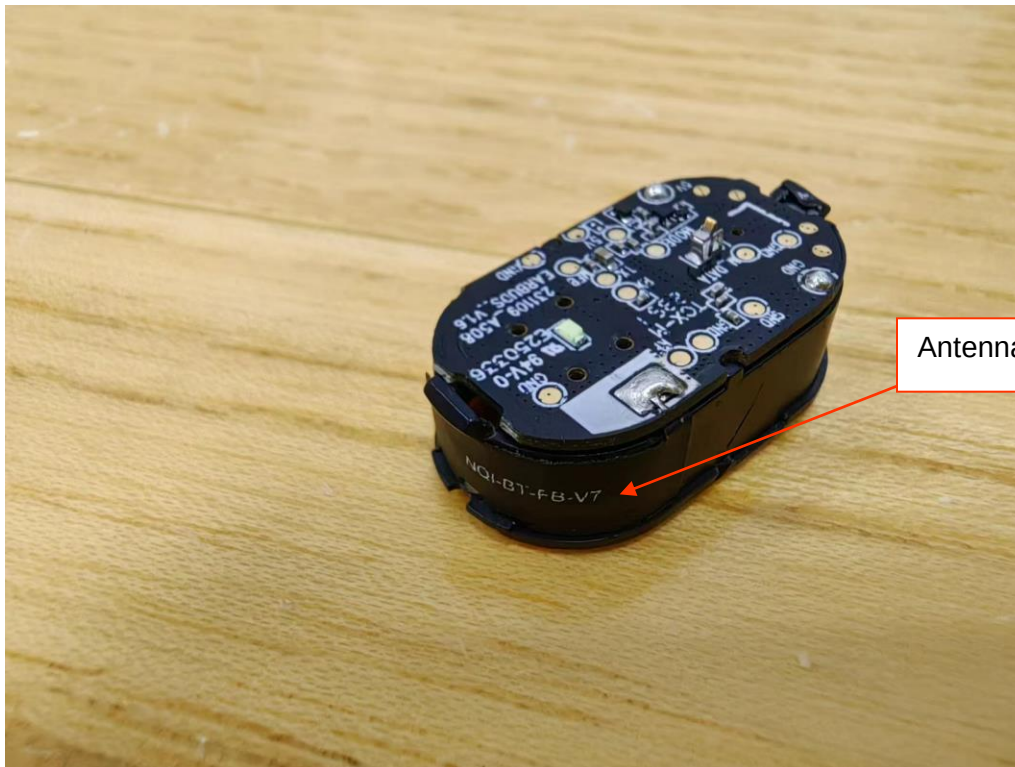
Internal View of EUT-4-L
