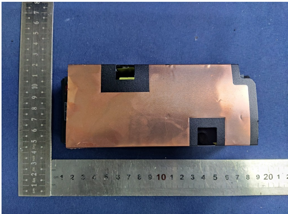
5.8G SRD antenna 5729-5845MHz
