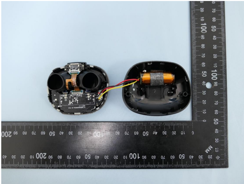
(28) EUT Photo_ Charging Box
