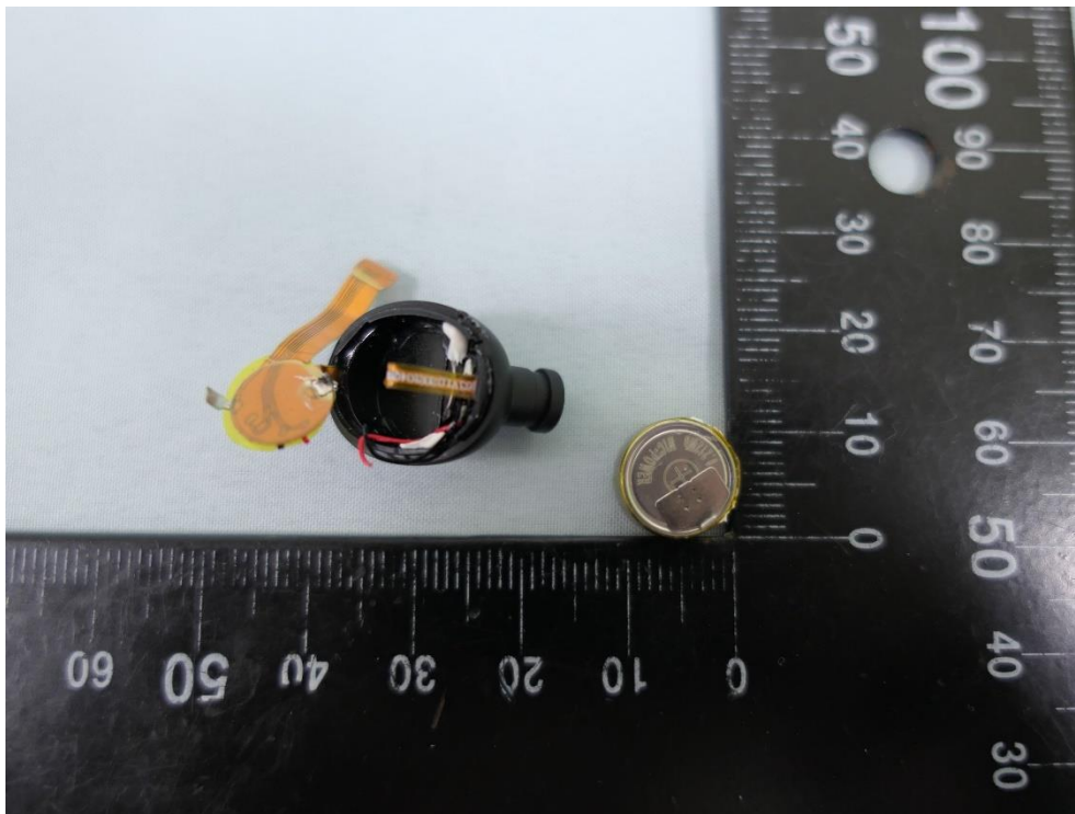
(17) EUT Photo_Right Ear
