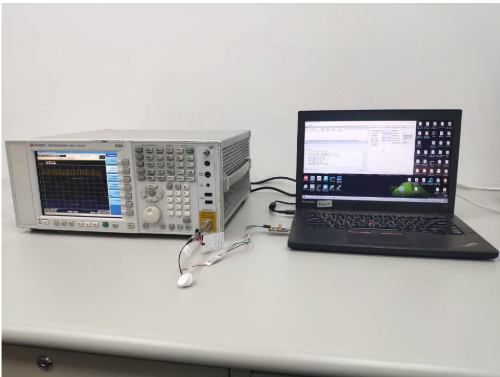
Description: Conducted Emission Test Setup _Right Ear
