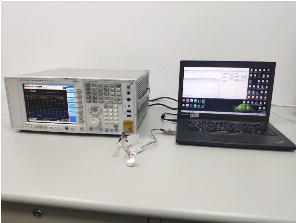
Description: Conducted Emission Test Setup _Left Ear
