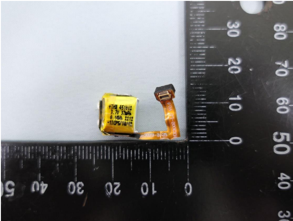
(6) EUT Photo_Left Ear(Battery:Zhongshan Tianmao Battery Co.,Ltd.)
