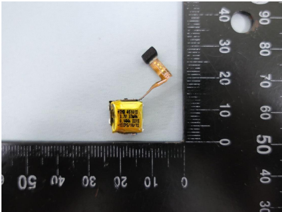
(16) EUT Photo_Right Ear(Battery:Zhongshan Tianmao Battery Co.,Ltd.)
