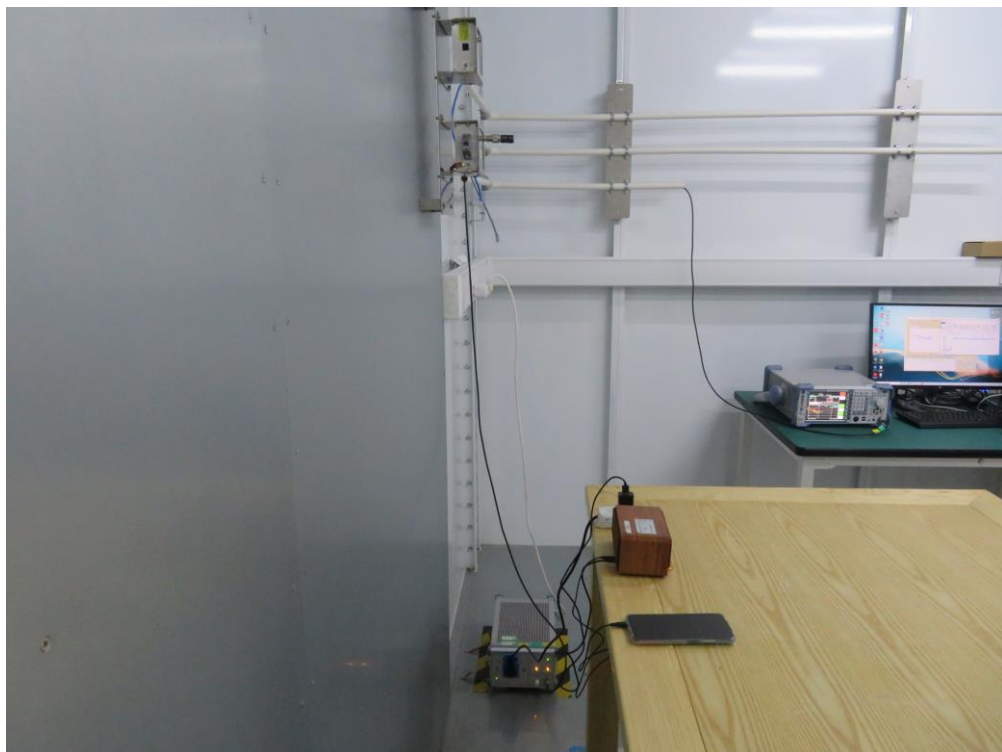
Description: AC Mains Back View of Conducted Emission Test Setup
